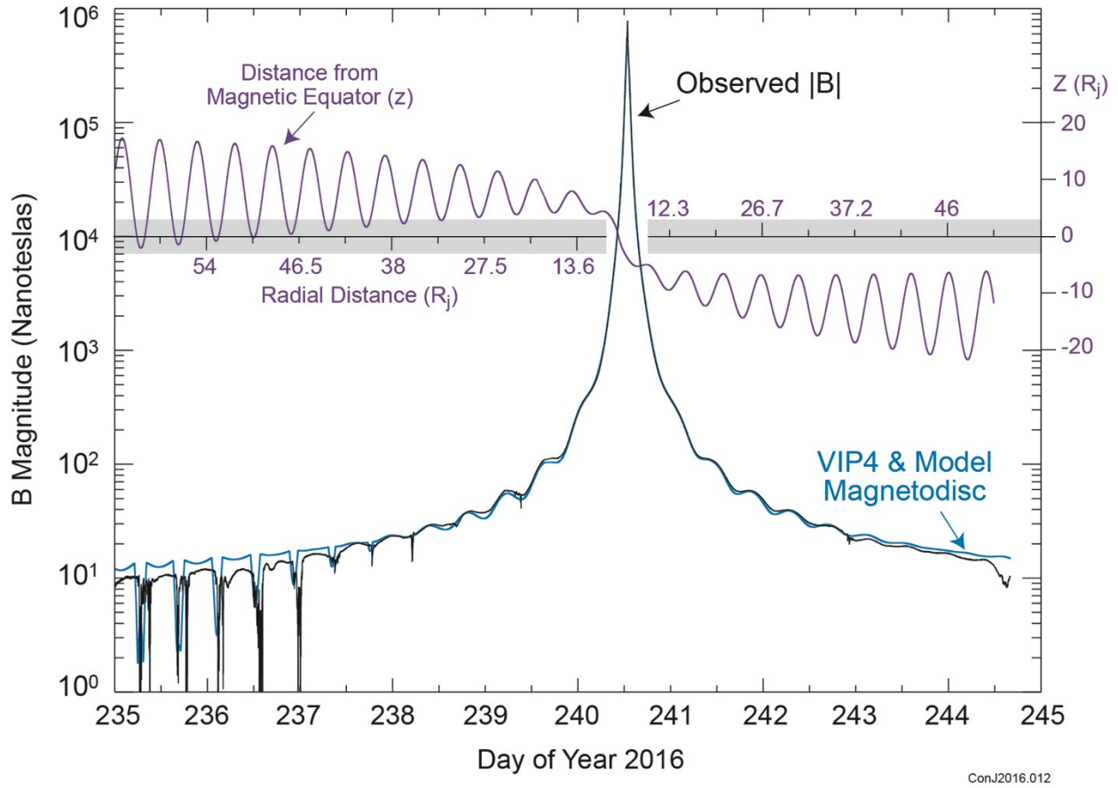
Fig. 1.: Measured magnetic field magnitude (black, solid) and distance from the magnetic equator (purple) as a function of time and distance from Jupiter during Juno’s first perijove pass, compared to a model (blue) that combines the planetary magnetic field (VIP4 spherical harmonic [10] model) with that of the magnetodisc, a system of azimuthal currents confined to within \sim 3 R_j of the magnetic equator (shaded region). The magnetic field magnitude increases by over six orders of magnitude on approach to perijove, where a field of 7.776 G was observed.
