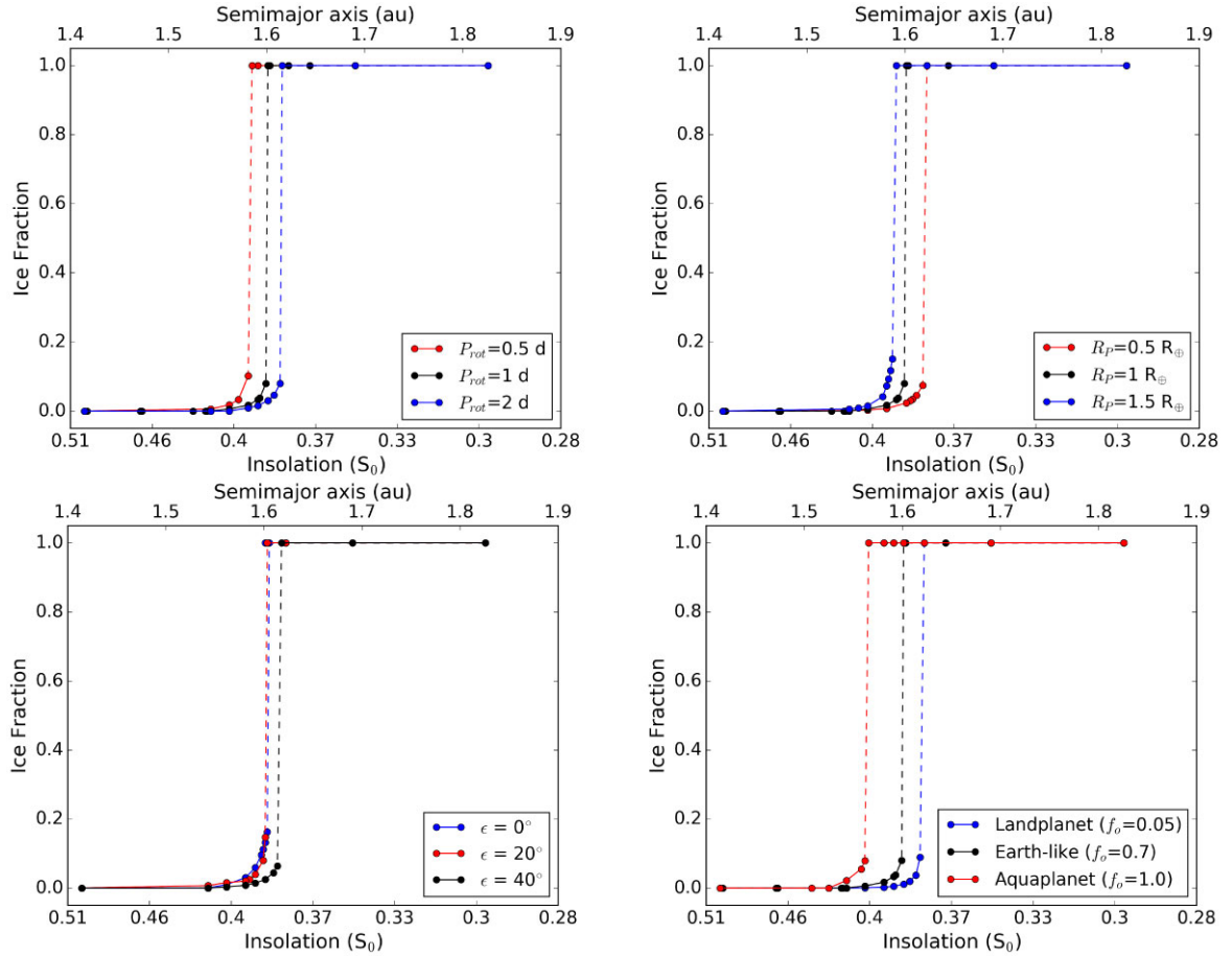
Figure 14. Dependence on planetary parameters of the fractional ice coverage calculated at the outer edge of the HZ. The results were obtained for a cloud-free Earth-like planet with a \text{CO}_2 -dominated, maximum greenhouse atmosphere, the remaining parameters being fixed to Earth values; only the solutions obtained with warm initial conditions ( T_0 = 300 K) are shown (see Section 4.5). Top left panel: rotation period, P_{\text{rot}} ; top right panel: planet radius, R_p ; bottom left panel: axis obliquity, \epsilon ; bottom right panel: geography.
