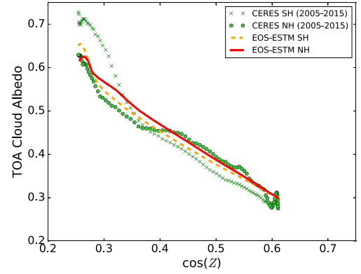
Figure 6. Cloud albedo versus \mu = \cos Z for the present-day Earth (Northern and Southern hemispheres). Dark green circles and crosses: observational data obtained from equation (10) for the Northern and Southern hemisphere, respectively. Red-solid and orange-dashed lines: ESTM predictions obtained by converting to TOA values the cloud albedo calculated from equation (12) for the Northern and Southern hemisphere, respectively.
