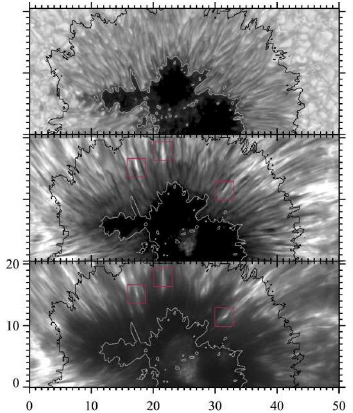
Fig. 9. Filtergram images of the continuum around the Fe I 630.1 nm line ( top ), the blue wing of the Ca II 854.2 nm line at -0.021 nm ( middle ), and the blue wing of the Ca II K line at -0.024 nm ( bottom ). Pink squares show the position of penumbral microjets in the middle and bottom panels. Axes are in arcseconds. Contours outline the inner and outer boundaries of the penumbra. Adapted from Esteban Pozuelo et al. (2019).
