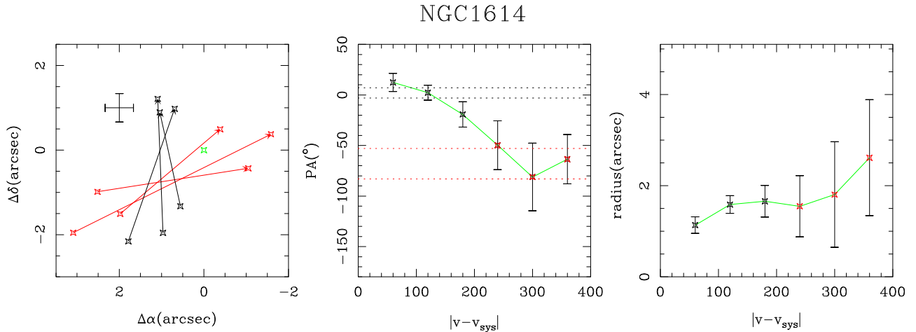
Fig. 3. Centroids of CO(1–0) emission in NGC 1614 (in [\Delta\alpha, \Delta\delta] -units) derived with a velocity resolution of 60 \text{ km s}^{-1} , using a power law of the flux as weighting function with index n = 1/2 , are displayed in the left panel . Emission centroids calculated for velocity channels that are equidistant from v_{\text{sys}} (i.e., with a common |v - v_{\text{sys}}| -offset) are connected to visualize the change of PA, defined for the redshifted component of the connected centroids and measured east from north, as a function of velocity ( middle panel ). We also plot the change in the average radius r , defined as half of the mutual distance from the connected centroids, as a function of velocity ( right panel ). Red color is used for velocity channels of the line wing and black color for the line core. The dotted black (red) line in the middle panel identifies the \pm 1\sigma range around the average PA of the disk as derived inside the line core (line wing): \text{PA}_{\text{core}} = 2 \pm 5^\circ ( \text{PA}_{\text{wing}} = -68 \pm 15^\circ ). The green marker in the left panel identifies the dynamical center. Error bars as a function of velocity channel are shown in the middle and right panels. Error bars in the left panel are for the line core.
