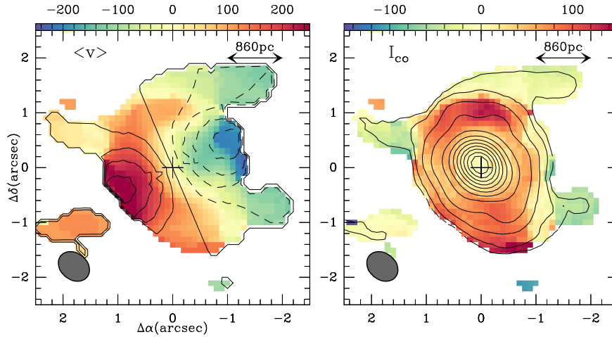
Fig. 15. Same as Fig. 7, but showing here the comparison between the CO(2–1) observations and the best-fit model in IRAS 17208-0014. Contours in the left panel span the range -200 km s^{-1} to 200 km s^{-1} in steps of 50 km s^{-1} . The CO(2–1) intensity contours in the right panel are as in the left-hand panel of Fig. 12. Color scales in both panels are as shown.
