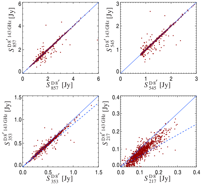
Fig. A.1. Comparison of the flux densities of the PHZ source candidates (at 8') computed on the cleaned maps obtained using the Planck 143 GHz map ( S_v^{D8'}{}^{143} ) or the SMICA CMB component map ( S_v^{D8'} ) as a CMB template during the cleaning processing. The blue line provides the 1:1 reference. The dashed line gives the expected attenuation coefficients of 10 % at 353 GHz and 40 % at 217 GHz due to extragalactic foreground contamination of the CMB template.
