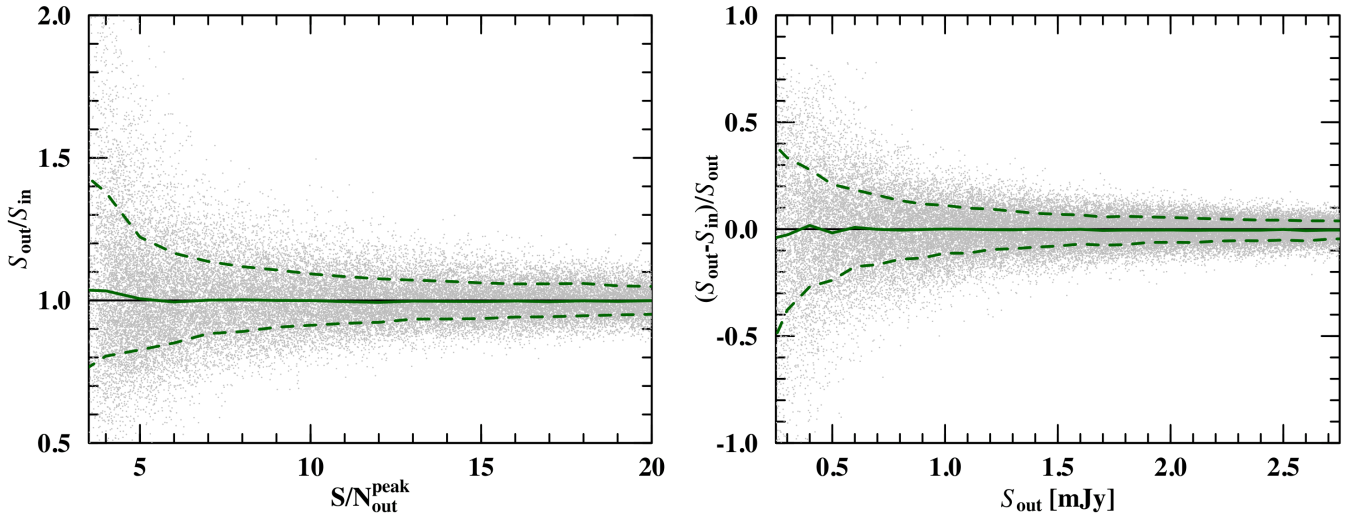
Fig. 9. Ratio of the output over input flux densities ( S_{\text{out}}/S_{\text{in}} ) as a function of the output detection S/N^{\text{peak}} ( S/N^{\text{peak}} ) from PyBDSF, measured as the peak flux density over the local rms noise ( left panel ), and flux density accuracy ( (S_{\text{out}} - S_{\text{in}})/S_{\text{out}} ) as a function of the output flux density ( S_{\text{out}} ) measured with the aperture photometry methodology ( right panel ) for simulated sources with sizes ranging 0'.1-0'.4 FWHM. The distribution of the whole set of simulations is shown as gray symbols with their sliding median and standard deviation in solid and dashed green, respectively.
