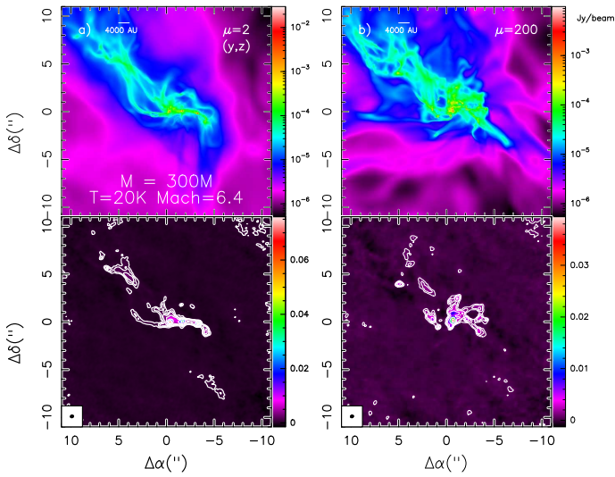
Fig. 9. Simulations of the gravitational collapse of a 300 M_{\odot} collapsing clump, with gas temperature T = 20 K, and Mach number M \sim 6.4 . a) : model predictions for the strongly magnetised case, \mu = 2 . In the top panel, we show the direct outcome of the simulations, while the same image processed with the CASA simulator is shown in the bottom panel. The first contour is 0.6 \text{ mJy beam}^{-1} as in Fontani et al. (2016), roughly 3 times the 1\sigma rms of most images). The steps are 1.2, 2, 5, 10, 30 and 50 \text{ mJy beam}^{-1} . b) : same as a) for the weakly magnetised case, \mu = 130 . These simulations have the same set of initial parameters as those discussed in Fontani et al. (2016), but we have post-processed and analysed those at which the star formation efficiency (SFE) is 15%, while in Fontani et al. (2016) we analysed the time at which the SFE matched that of IRAS 16061–5048c1 ( \sim 30\% ).
