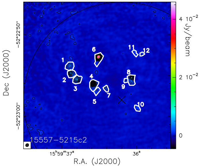
Fig. A-4. Same as Fig. A-1 for 15557–5215c2. The first contour level, and the step, is 7.8 \times 10^{-4} \text{ Jy beam}^{-1} , corresponding to the 3\sigma rms noise level ( 1\sigma \sim 2.6 \times 10^{-4} \text{ Jy beam}^{-1} ).
