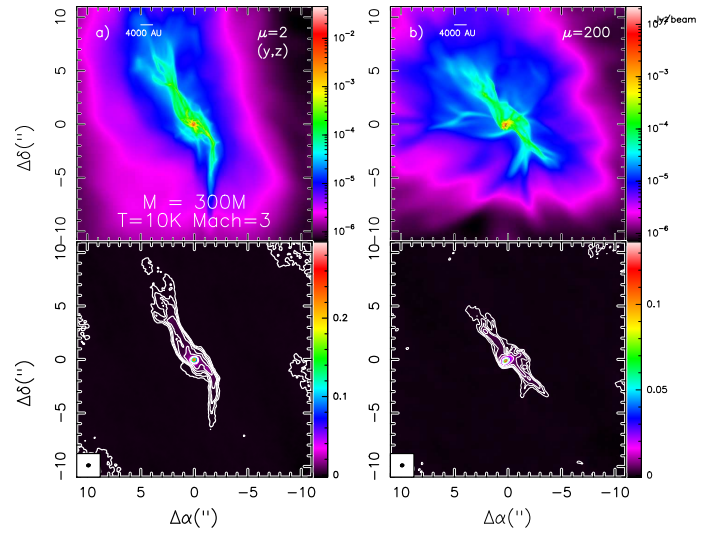
Fig. 10. Same as Fig. 9 for a clump with Mach number M \sim 3 .
