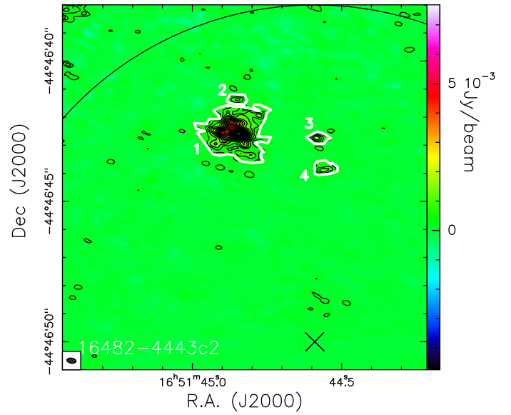
Fig. A-6. Same as Fig. A-1 for 16482–4443c2. The first contour level, and the step, is 3 \times 10^{-4} \text{ Jy beam}^{-1} , corresponding to the 3\sigma rms noise level ( 1\sigma \sim 1 \times 10^{-4} \text{ Jy beam}^{-1} ).
