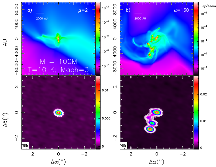
Fig. 8. Simulations of the gravitational collapse of a 100 M_{\odot} collapsing clump, with gas temperature T = 10 K, and Mach number M \sim 3 . a) : model predictions for the strongly magnetised case, \mu = 2 . In the top panel, we show the direct outcome of the simulations, while the same image processed with the CASA simulator is shown in the bottom panel (first contour and step is 0.3 \text{ mJy beam}^{-1} ). b) : same as a) for the weakly magnetised case, \mu = 130 .
