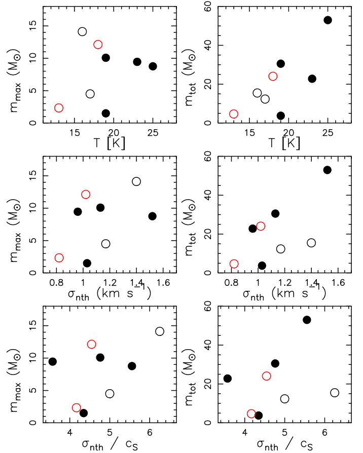
Fig. 5. Maximum and total mass of the fragments ( m_{\text{max}} and m_{\text{tot}} , respectively) as a function of the clump gas temperature ( T ), the non-thermal velocity dispersion ( \sigma_{\text{nth}} ), and the ratio between \sigma_{\text{nth}} and the sound speed ( c_s ), i.e. the Mach number. The typical uncertainties on the masses, mainly due to the mass opacity coefficient, can be up to a factor 2–3 (see Sect. 4.1).
