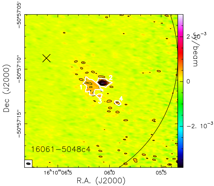
Fig. A-5. Same as Fig. A-1 for 16061–5048c4. The first contour level, and the step, is 3 \times 10^{-4} \text{ Jy beam}^{-1} , corresponding to the 3\sigma rms noise level ( 1\sigma \sim 1 \times 10^{-4} \text{ Jy beam}^{-1} ).
