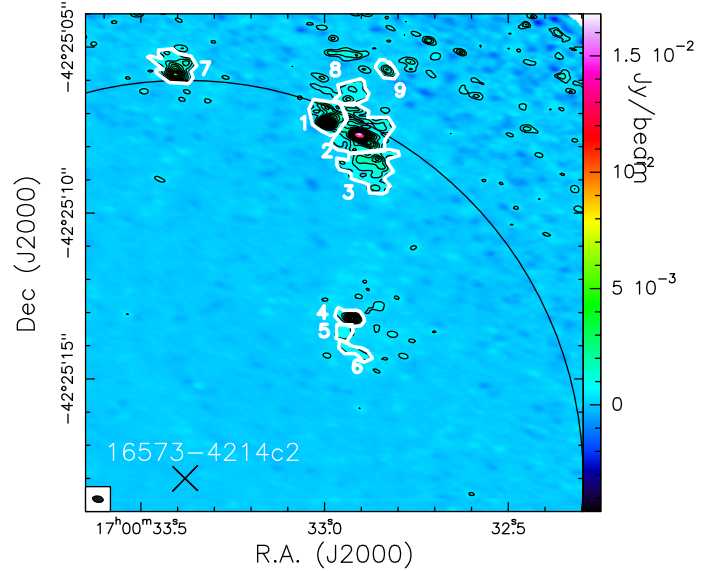
Fig. A-7. Same as Fig. A-1 for 16573–4214c2. The first contour level, and the step, is 4.8 \times 10^{-4} \text{ Jy beam}^{-1} , corresponding to the 3\sigma rms noise level ( 1\sigma \sim 1.6 \times 10^{-4} \text{ Jy beam}^{-1} ).
