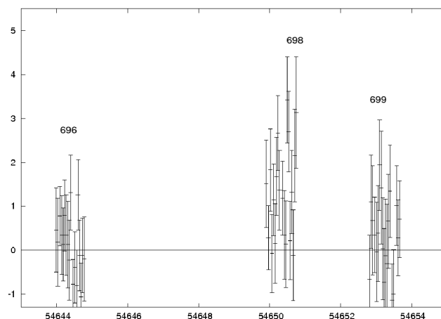
Figure 8. IBIS/ISGRI light curve (18–60 keV) at ScW level of IGR J12341–6143 covering the period from revolution 696 to 699.
