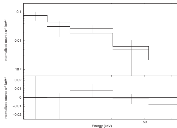
Figure 9. IBIS/ISGRI spectrum of IGR J12341–6143 extracted during the outburst, it is best fitted by a bremsstrahlung model. The lower panel shows the residuals from the fit.
