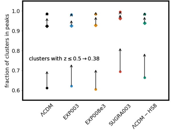
Figure 11. Fraction of clusters for a space-based analysis with M_{200} \geq 10^{14} M_{\odot} h^{-1} and z \leq 0.5 in peaks with convergence values above f_{\sigma} = 2, 3, and 5 from top to bottom data points, respectively. The arrow on each data point shows the corresponding fraction of clusters in peaks when we select systems with z \leq 0.38 – the peak of the lensing kernel for z_s = 1.12 .
