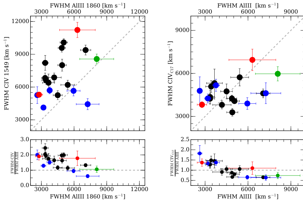
Fig. 4. Relation between the FWHM \text{AIII}\lambda 1860 and FWHM \text{CIV}\lambda 1549 before ( left ) and after ( right ) Coatman et al. (2017) correction. Dashed gray line corresponds to the 1:1 line. Bottom panels : ratio between the FWHM \text{CIV}\lambda 1549 and \text{AIII}\lambda 1860 . Colors are the same as the Figs. 2 and 3.
