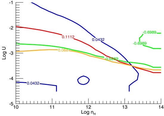
Fig. 7. Isocontours in the plane \log of ionization parameter ( U ) versus \log of hydrogen density ( n_{\text{H}} ) from CLOUDY simulations for the line intensity ratios \text{AlIII}\lambda 1860/\text{SiIII}\lambda 1892 (blue), \text{HeII}\lambda 1640/\text{CIV}\lambda 1549 (green), \text{CIV}\lambda 1549/\text{AlIII}\lambda 1860 (yellow), \text{CIV}\lambda 1549/\text{SiIII}\lambda 1892 (red) using Z = 100 Z_{\odot} . Labels report the median values of the intensity ratios for the objects of the GTC-xA sample.
