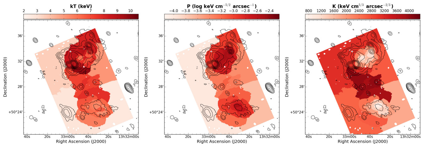
Figure 8. Thermodynamical properties of the ICM in A1758 with overlaid the LOFAR contours of Fig. 1. Images depict projected values of temperature (left), pressure (centre), and entropy (right). The temperature error map and a lower S/N temperature map are reported in Appendix A.
