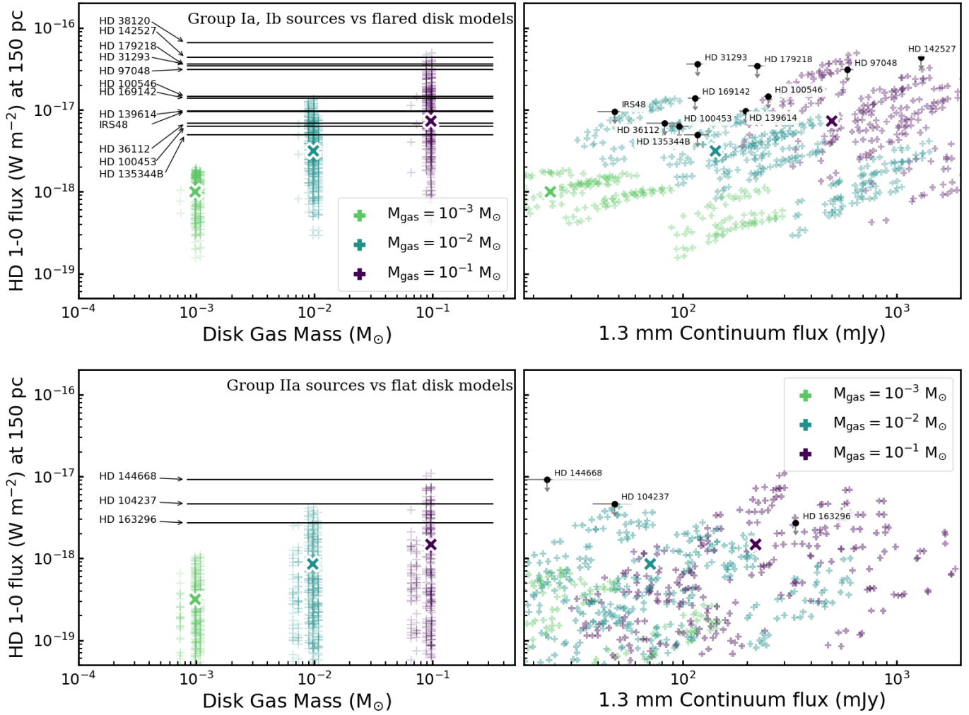
Fig. 2. Distance-normalised 3\sigma upper limits on HD 112\ \mu\text{m} line flux for the disc sample (black lines and circles) compared with our grid of DALI disc models (coloured crosses). Highlighted crosses show the HD 112\ \mu\text{m} line flux of our fiducial model. The top panels show the group I sources compared to models with flaring angle \psi = 0.3 . The bottom panels show the group II sources compared to models with \psi = 0.0 . Left : models are separated based on gas mass. Right : HD 1–0 upper limits set against 1.3 mm continuum fluxes for both observations and models.
