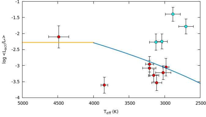
Fig. 8: \log \langle L_{acc}/L_* \rangle vs T_{eff} for all our targets. The cyan dots represent accretors, and the red dots represent chromospherically-dominant targets. The lines indicate the limit below which the chromospheric activity for a star is dominant (Manara et al. 2017b), for two regimes of stars with T_{eff} \leq 4000 K (the diagonal blue line) and those with T_{eff} \geq 4000 K (the horizontal orange line).
