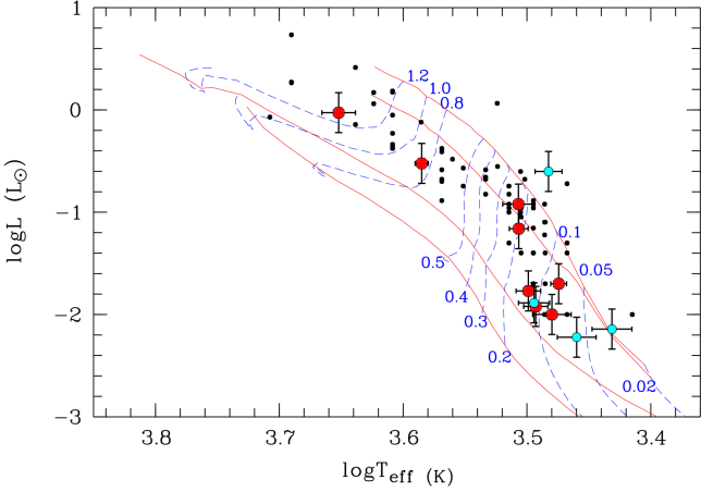
Fig. 3: \log L_*(L_\odot) vs \log T_{\text{eff}} (K) diagram for all our targets (cyan and red dots represent accretors and non-accretors, respectively), together with the previously characterized Lupus members (black dots, Alcalá et al. 2019, sub-luminous objects are not plotted). Blue dashed lines represent evolutionary tracks of Baraffe et al. (2015) for stars with masses indicated by the number (in M_\odot ) next to the top or bottom of each track. The red lines indicate isochrones calculated with the same models at ages of 1, 3, 30 Myrs, and 10 Gyrs, from the right to the left.
