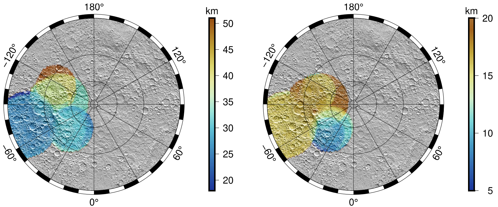
Figure S24 Maps of the lateral variations of the (left) crustal thickness and (right) its uncertainty in a polar stereographic projection from 30°N-latitude. This map is obtained by assuming surface loads only. Grey colors show regions where the localized admittance spectra do not allow to constrain the crustal density.
