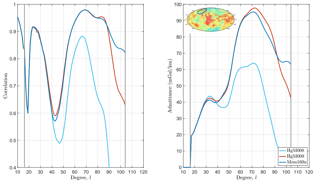
Figure S8 Gravity/topography ( left ) correlation and ( right ) admittance spectra on a local spherical cap centered at 60^\circ\text{N} -latitude and 290^\circ\text{E} -longitude with a radius of 20^\circ , a concentration factor of 99.9%. The gravity fields used in this localized admittance analysis are HgM008 ( cyan ) [5], HgM009 ( red ) and Mess160a ( blue ) [6]. Vertical gray lines show the degrees range between L_{win} and l_{max} - L_{win} , which is equal to l_{DS}=104 (Figure S1).
