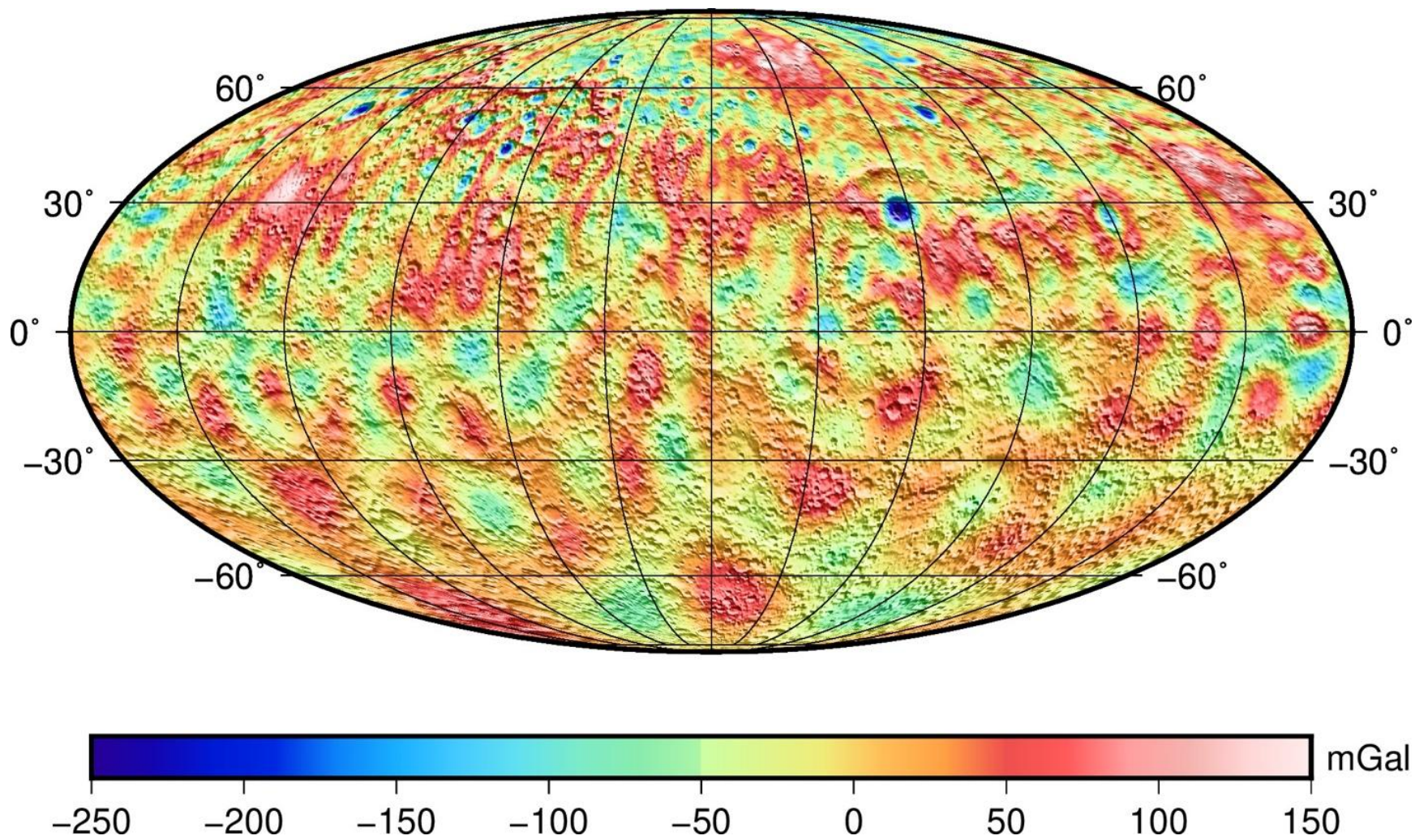
Figure S4 Global map of the free-air gravity anomaly (mGal) from gravity field HgM009 in a Mollweide projection centered on 0° longitude. The shaded topographic relief is based on the (USGS) map by [4].
