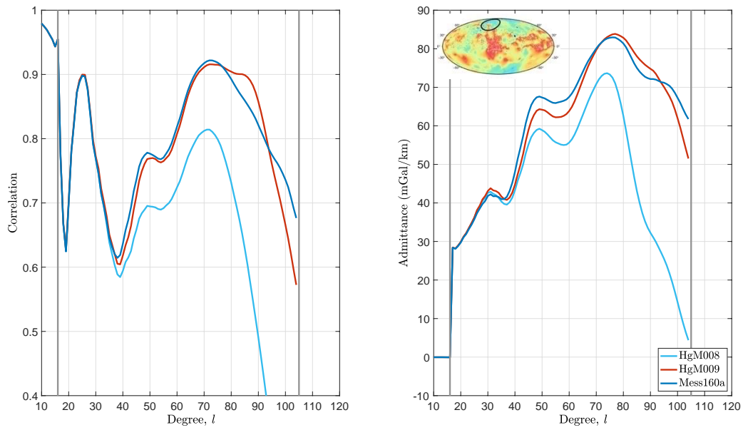
Figure S9 Gravity/topography ( left ) correlation and ( right ) admittance spectra on a local spherical cap centered at 64^{\circ}\text{N} -latitude and 319^{\circ}\text{E} -longitude with a radius of 20^{\circ} , a concentration factor of 0.999. The gravity fields used in this localized admittance analysis are HgM008 ( cyan ) [5], HgM009 ( red ) and Mess160a ( blue ) [6]. Vertical gray lines show the degrees range between L_{win} and l_{max} - L_{win} , which is equal to l_{DS}=105 is given by the degree strength map (Figure S1).
