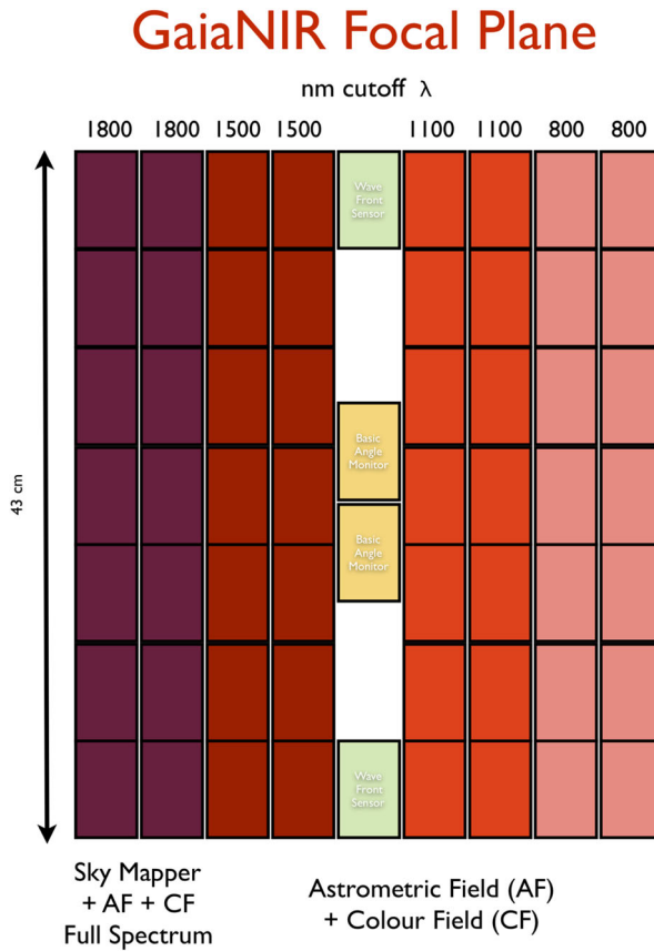
Fig. 4 Proposed focal plane array and filter bands used in the GaiaNIR CDF study (see page 203 in https://sci.esa.int/s/8a65kZA ). The array consists of 60 NIR detectors, arranged in 7 across-scan rows and 9 along-scan strips (out of which 8 are for the astrometric/photometric field, divided into 4 photometric fields (i.e. 4 different cut-off wavelengths each starting from \sim 400 nm). The new array is less than half the size of Gaia's
