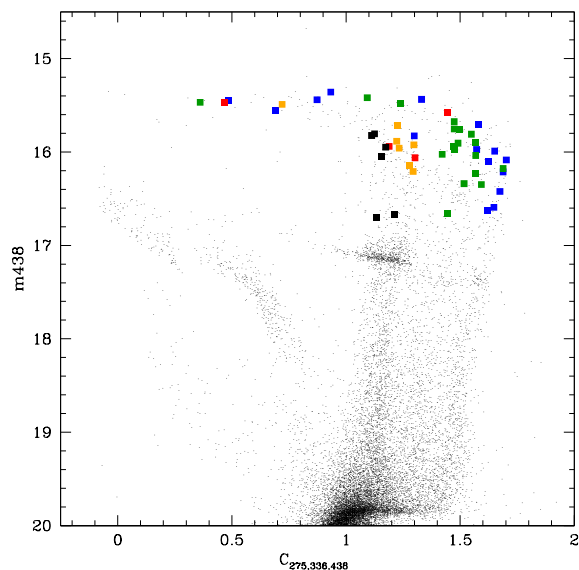
Fig. 9. Diagram using the pseudo-colour C_{275,336,438} against F438W . The stars in our spectroscopic sample are plotted using larger, filled symbols and adopting the same colour scheme of previous figures (P1: blue, P2: green, I1: red, I2: orange, and E: black).
