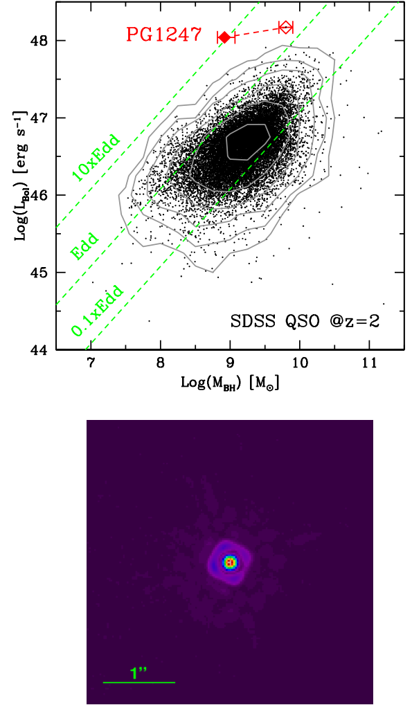
Fig. 1. Top: L_{\text{bol}} and M_{\text{BH}} for the 1.8 < z < 2.2 SDSS QSO sample (black points and gray contours). Values for PG1247 from SDSS (Shen et al. 2011) and from Trevese et al. (2014) are shown with empty and filled red diamonds, respectively. Dashed green lines mark different \lambda_{\text{Edd}} values. Bottom: 4'' \times 4'' HST-NICMOS image of PG1247 (filter F160W ). The 1'' scale is shown.
