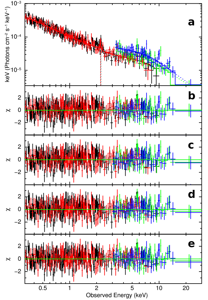
Fig. 6. Panel a) unfolded data and model for the best fit obtained with model 1. Panels b)–e) delta \chi for model 1, 2, 3, and 4, respectively. In all panels XMM-Newton pn data are in black, MOS1+2 in red, NuSTAR module A in green, and B in blue.
