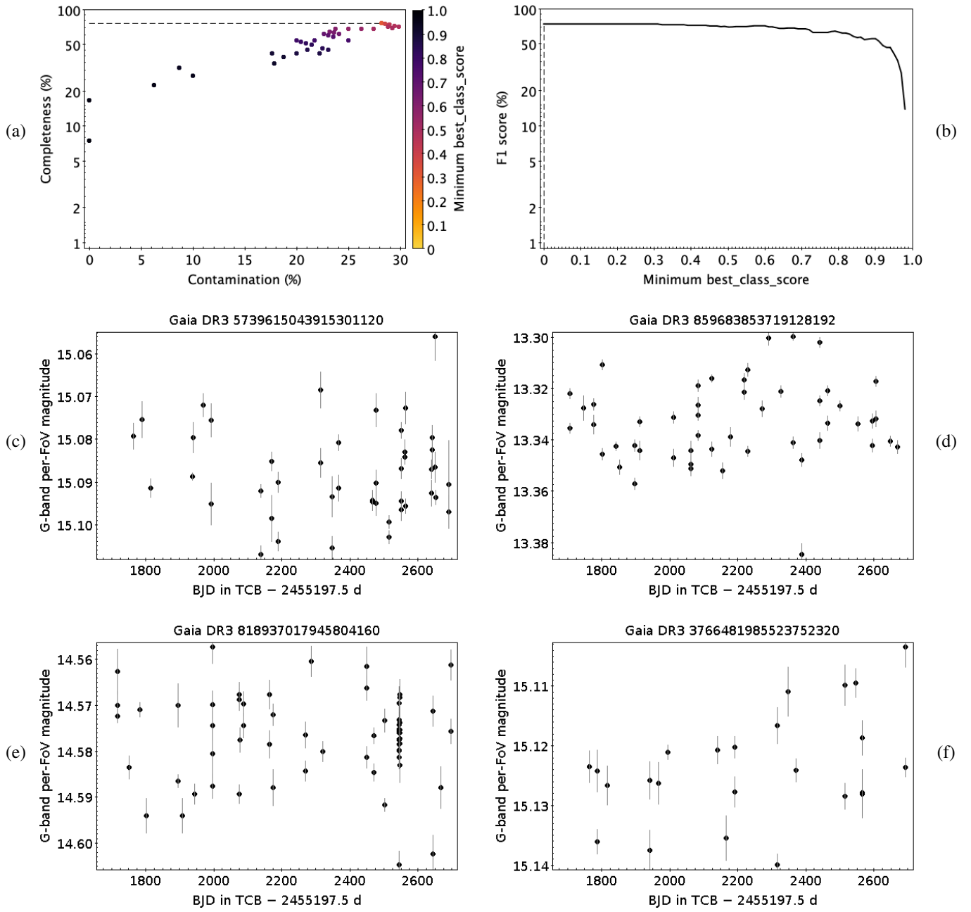
Fig. E.54. Same as Fig. E.3, but for SDB. Given the multiple significant periods of SDB stars, only time series are shown in panels (c)–(f).
