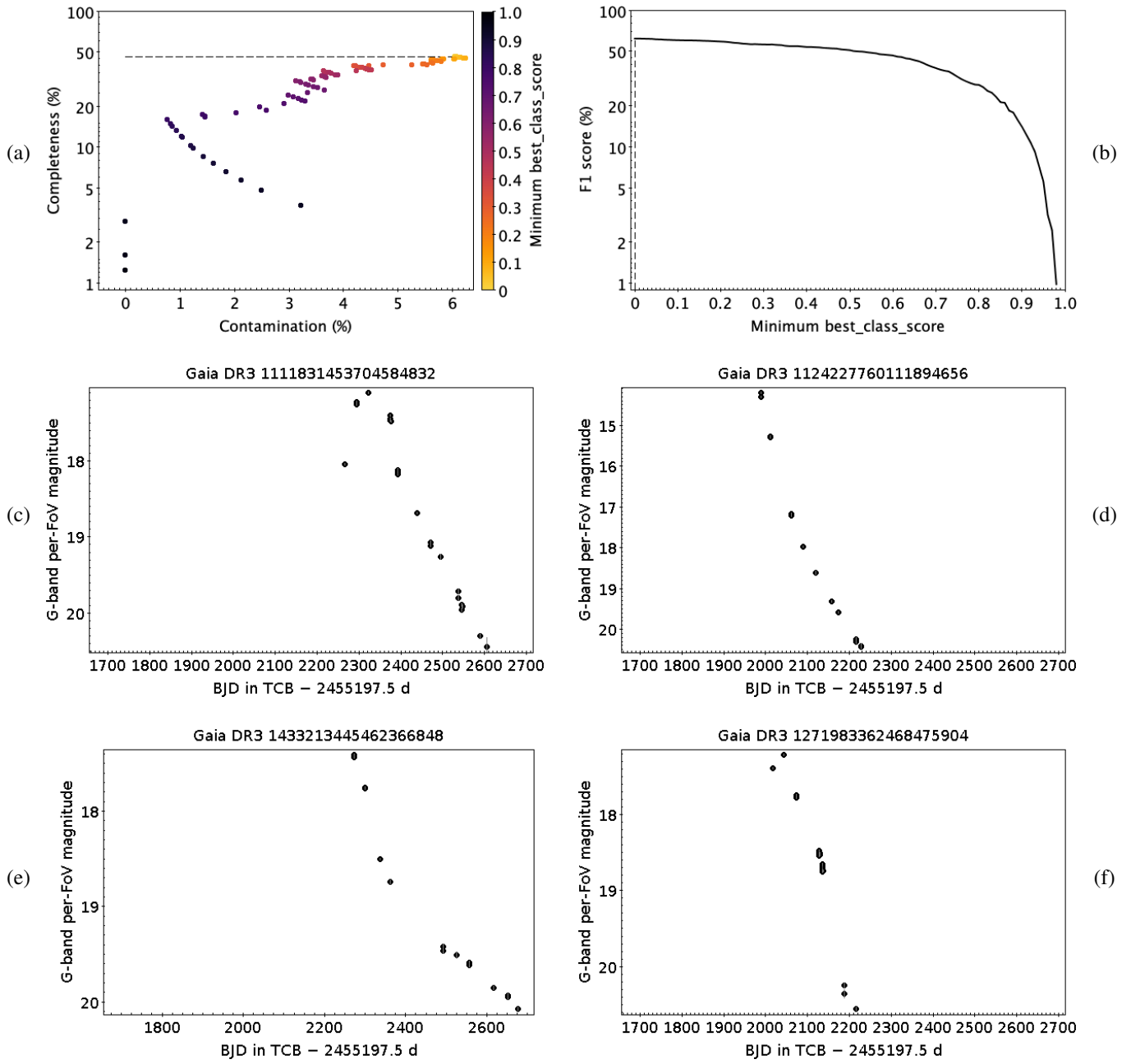
Fig. E.57. Same as Fig. E.3, but for SN.
