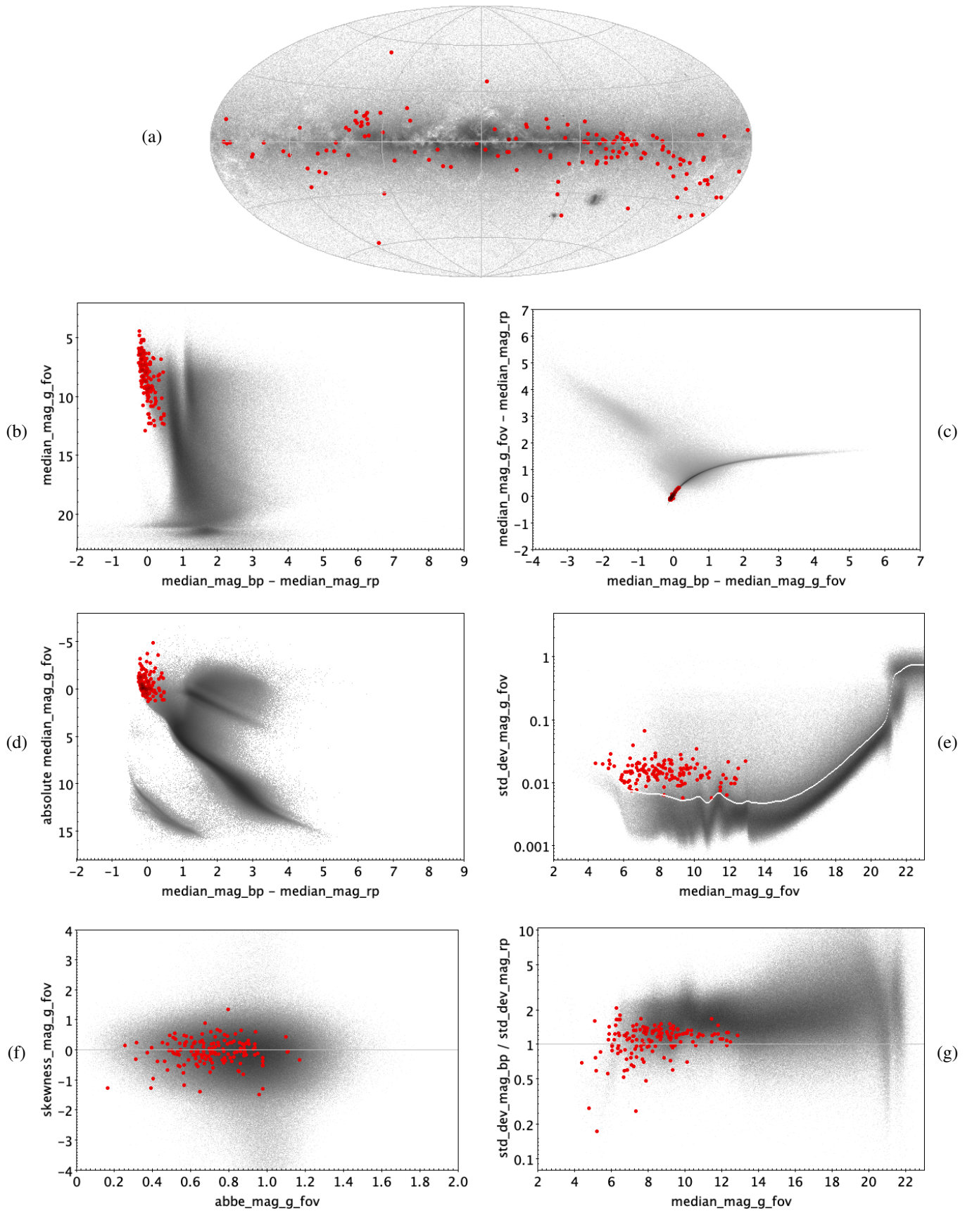
Fig. E.61. SPB: 149 training sources.
