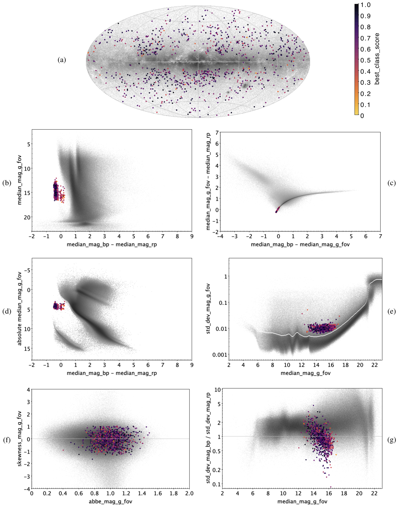
Fig. E.53. SDB: 893 classified sources.
