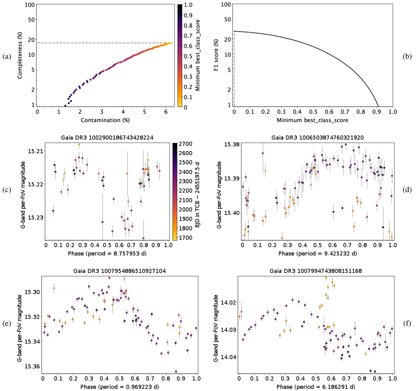
Fig. E.60. Same as Fig. E.3, but for SOLAR_LIKE.
