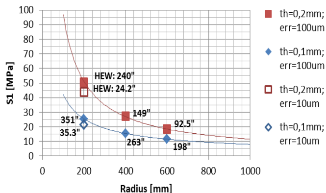
Figure 3: Maximum stress in a flat glass integrated with cold slumping approach after the vacuum release, and expected HEW of the integrated samples
