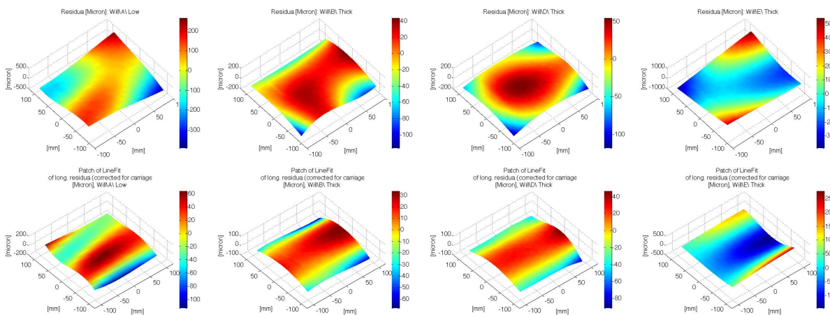
Figure 4: The residua with respect to a plane and along the vertical direction as measured on the four samples considered.
