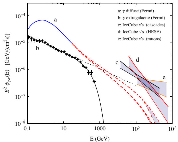
FIG. 16. Curve a shows the diffuse Galactic gamma-ray flux observed by Fermi (solid line) and the extrapolations calculated under the assumptions of a factorized (dashed line) and nonfactorized (dot-dashed line) emission. The Fermi measurement of the extragalactic gamma-ray flux [58] is shown by data points and with line ( b ) that is a fit with the functional form of a power law with an exponential cutoff (the dashed line shows the fit extrapolation without the cutoff). The shaded regions c , d and e show estimates of the neutrino flux obtained by IceCube under the assumption of an isotropic extragalactic flux [19]. All fluxes are integrated over the entire sky.
