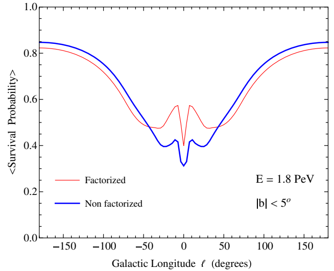
FIG. 14. Top panel: Longitude distribution of the gamma-ray flux at E = 1.8 PeV, integrated in the latitude range |b| < 5^\circ . The flux is shown for both our models (factorized and nonfactorized emissions), including and neglecting the effects of absorption. Bottom panel: Average survival probability for gamma rays of energy E = 1.8 PeV, averaged in the latitude interval |b| < 5^\circ , as a function of the Galactic longitude, according to our two models.
