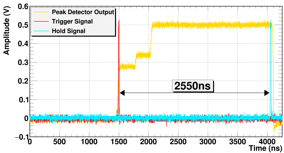
Figure 4. Peak detector analog output when an electronic signal with multiple pulses (having different amplitudes) is injected. The yellow curve shows the analog signal of the peak detector. The red and blue curves are the trigger and hold signals, injected from the pulse generator. As evident, after the injection of the highest amplitude pulse, the peak detector output stays constant, without any appreciable decay in the considered time intervals, until the falling edge of the Hold signal.
