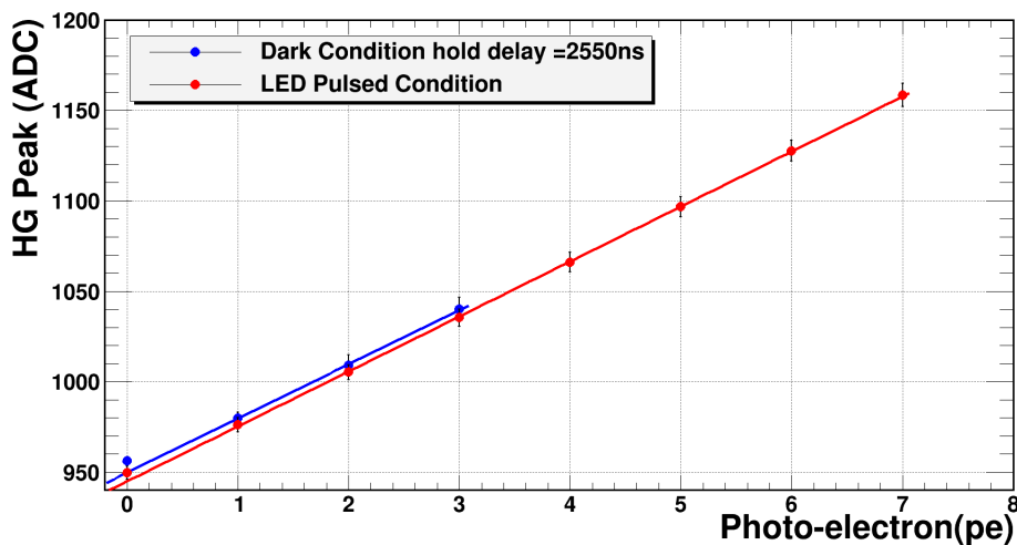
Figure 10. Values in ADC unit of the peaks of the spectrum distribution as a function of the number of photo-electrons, for the case of the spectrum obtained keeping the sensor in dark (blue points) and with the external pulsed light (red points).
