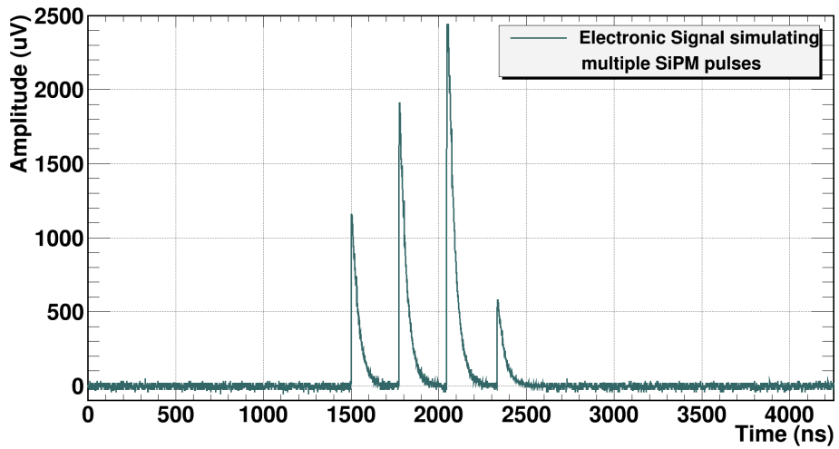
Figure 3. Electronic signal injected into an ASIC channel to study the peak detector output in presence of multiple SiPM pulses detected within short time distance.
