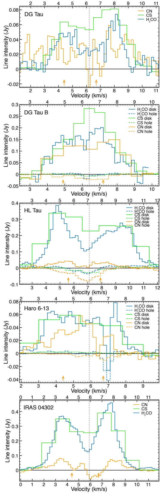
Fig. C.1. Spectral profile of \text{H}_2\text{CO} , CS, and CN for the full sample analyzed in this work. The profile is obtained over the disk region determined by the parameters of Table 3 (continuous lines) and in the inner region with dimmed flux (dashed lines). The vertical line indicates the systemic velocity constrained from the moment 0 map. The two arrows denote the wavelength of the CN blended lines (see Table 2). Both the horizontal and vertical scales of the various diagrams are different.
