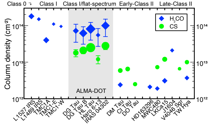
Fig. 6. CS and \text{H}_2\text{CO} column densities from this work compared with the literature. The symbol size reflects the dust disk mass scaling between 5 and 370 M_{\oplus} . The \text{H}_2\text{CO} estimates of Class 0 and I sources are from van 't Hoff et al. (2020); HD163296 and TW Hya from Carney et al. (2019); and all others from Pegues et al. (2020). All CS estimates are from Le Gal et al. (2019), except TW Hya, which is from Teague et al. (2018). Taurus sources (1–2 Myr old) are named early-Class II, while the older ones (>2 Myr) are late-Class II.
