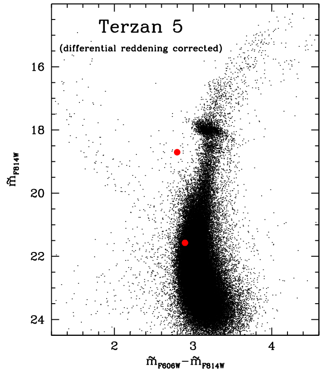
Figure 3. (m_{F814W}, m_{F606W} - m_{F814W}) CMD of Terzan 5 corrected for differential reddening (according to Massari et al. 2012). The position of the optical counterpart to EXO 1745-248, in the outburst and in quiescent states, is marked with large red circles.
