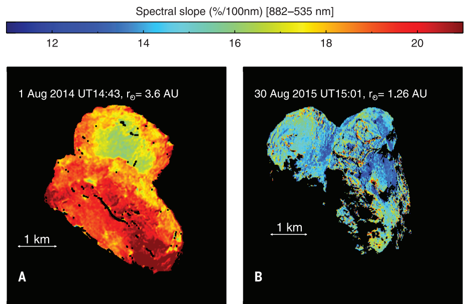
Fig. 1. Spectral slope evolution with heliocentric distance. The August 2014 image was corrected for the phase reddening from 10° to 70° using the coefficients published in (15) to match the viewing geometry on the right. See fig. S4 for the morphological regions context.
