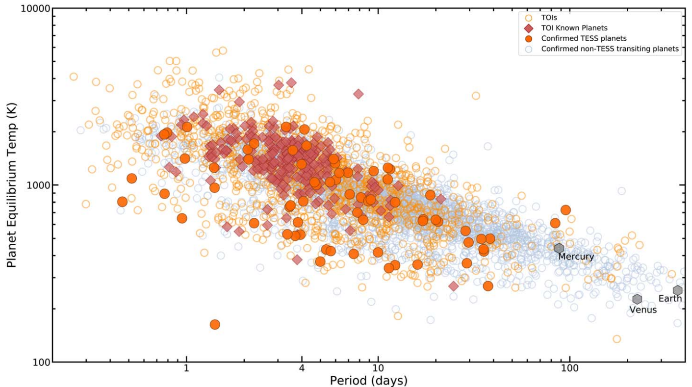
Figure 11. Orbital period vs. planet equilibrium temperature. The planet orbital period in days is on the horizontal axis, and the planet T_{\text{eq}} is on the vertical axis. The open orange circles are planet candidate TOIs that have not been confirmed. The filled orange circles are planets that are either confirmed with a mass measurement or validated by other means. The red diamonds are TOIs that were known planets prior to the TESS mission. The blue open circles are known planets from outside the TESS mission (NASA Exoplanet Archive, accessed 2020 October 8). Mercury, Venus, and Earth are visible in the bottom right. The TOI catalog has greatly increased the number of temperate short-period planet candidates available for follow-up.
