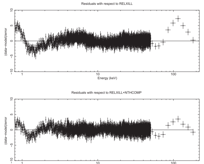
Figure 2. Residuals in units of sigma for the low/hard state spectra with respect to the model RELXILL (top panel) and RELXILL+NTHCOMP (bottom panel)
