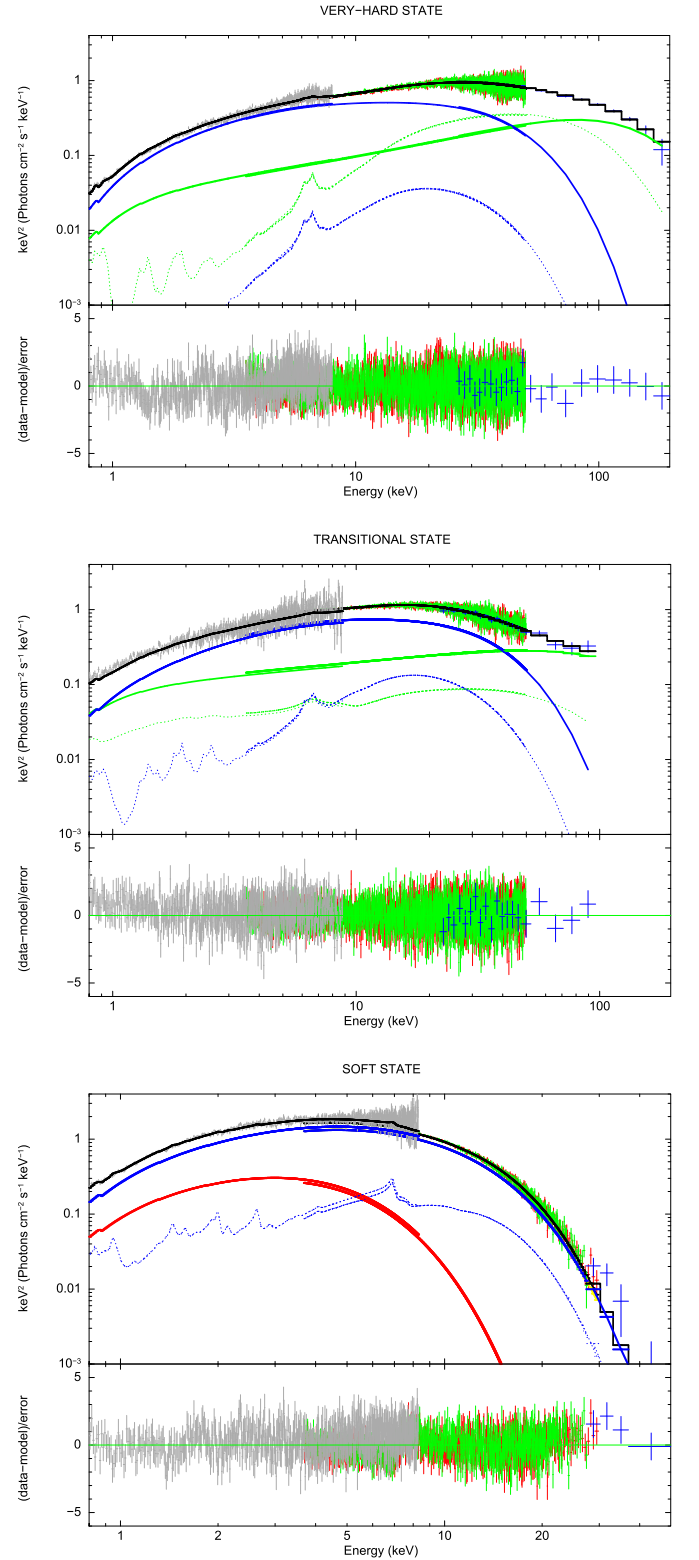
Figure 3. SWIFT/XRT, NuSTAR/FPMA and FPMB, and INTEGRAL/IBIS unfolded spectra and residuals in sigma rebinned for visual clarity for the very hard state (top panel), transitional state (middle panel), and high/soft state (bottom panel). Light gray points correspond to XRT data, red and green points correspond to FPMA and FPMB data, and blue points are IBIS data. For the very hard and transitional state we plot the spectral components of Model 2 and Model 1 for soft state. Red lines correspond to DISKBB components, blue lines to NTHCOMP components and its reflection component (blue dotted), green lines correspond to second NTHCOMP components and its reflection (green dotted).
