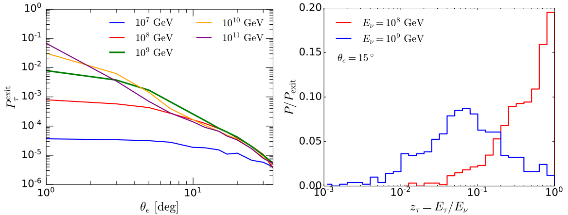
Figure 15. Left: The probability for a \nu_\tau to produce a \tau -lepton which exits the Earth, as a function of Earth emerging angle relative to horizontal, \theta_e = 1^\circ - 35^\circ , for incident neutrino energies of 10^7 , 10^8 , 10^9 , 10^{10} and 10^{11} GeV. The ALLM \tau -lepton energy loss model is used, as described in [148]. Right: The \tau -lepton energy distribution as a function of z = E_\tau/E_\nu for \tau -leptons exiting at an Earth emergence angle \theta_e = 15^\circ for E_\nu = 10^8 and 10^9 GeV.
