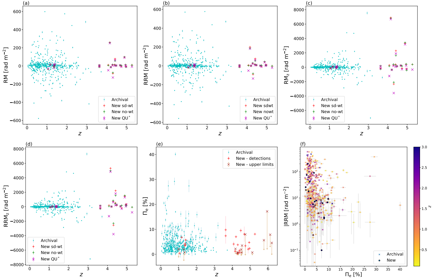
Figure 8. Rotation measures, polarization fractions, and redshifts compared against each other. From left to right top to bottom the panels are: (a) RM, (b) RRM, (c) RM_z , (d) RRM_z , (e) \Pi_e vs. z , and (f) |RRM| vs. \Pi_e colour coded by redshift. The blue circles are from the archival sample (with luminosity limits imposed), and for panels (a)-(d), the red pluses are the new data using the “sd-wt” weighting in the RM synthesis, the green pluses are the new data using the “no-wt” RM synthesis weighting, and the magenta crosses are the peak RMs from the QU fitting. In panel (e), the red pluses are the polarization fractions from those sources with RM detections, whereas the brown pluses are sources denoted as upper limits meaning there was no significant RM detection (those with flag=0 in Table 3). In panel (f) the crosses are the new sample with the RRM from the sd-wt RM synthesis values and the circles are the archival sources.
