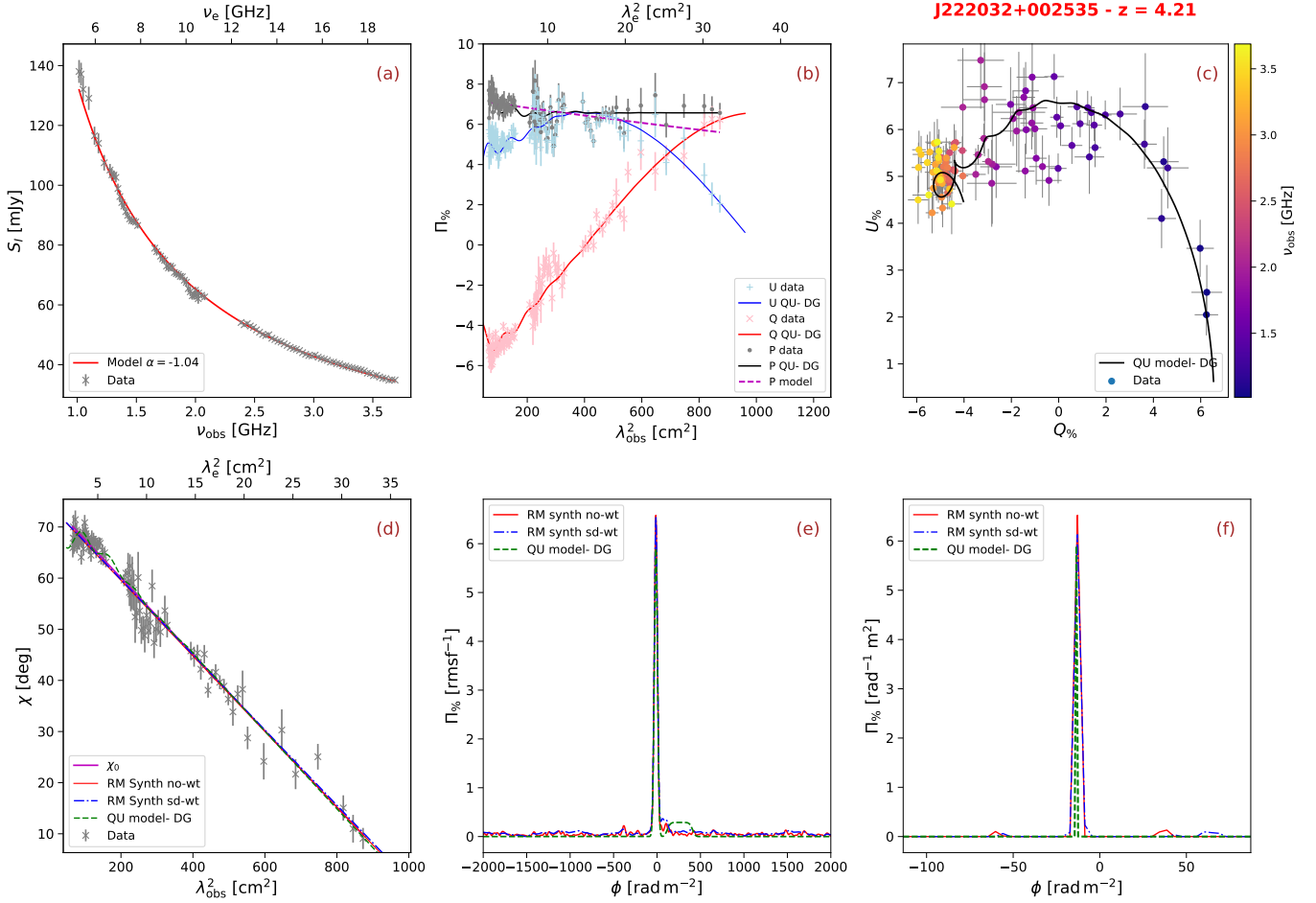
Figure 5. Spectra and Faraday dispersion functions for source J222032+002535. Panel (a) is the Stokes I spectrum vs frequency, with grey points showing the data and the red solid line showing the fitted model from eq.(2) or (3). Panel (b) shows the fractional Stokes Q (red) and U (blue) and P (gray) spectra vs \lambda^2 , with the points showing the image data and the lines showing the best-fit models from the QU fitting, the dashed purple line shows the best fit P model from eq.(5), (6), or (7). Panel (c) shows the fractional Stokes Q vs U with the solid line being the best-fit QU -fitting model and the colouring of the points showing the frequency. Panel (d) shows the polarization angle vs \lambda^2 , with the red solid and blue dot-dashed lines from the RM synthesis (eq. 8 and 9), the green dashed line from the QU fitting, and the purple solid line from the slope fitting. Panel (e) shows the fractional (cleaned) absolute value Faraday dispersion functions for “no-wt” (red solid) and “sd-wt” (blue dot-dashed) weighting and the QU -fitting (green dashed line) convolved with a Gaussian with width equal to the mean of the two RMSFs. Panel (f) shows the un-convolved (fractional) absolute value Faraday dispersion functions (or RMCLEAN clean components) from the “no-wt” RM synthesis (red solid), “sd-wt” (blue dot-dashed), and QU fitting (green dashed).
