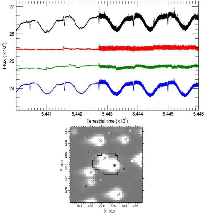
Fig. 6. Top : light curves in white, red, green, and blue (with the according colour code) of a false positive. Bottom : CoRoT image of the field around the target indicated by a star symbol (CID: 102779171, r -mag = 13.84) with the shape of the photometric mask overlaid and the location of nearby stars indicated with crosses.
