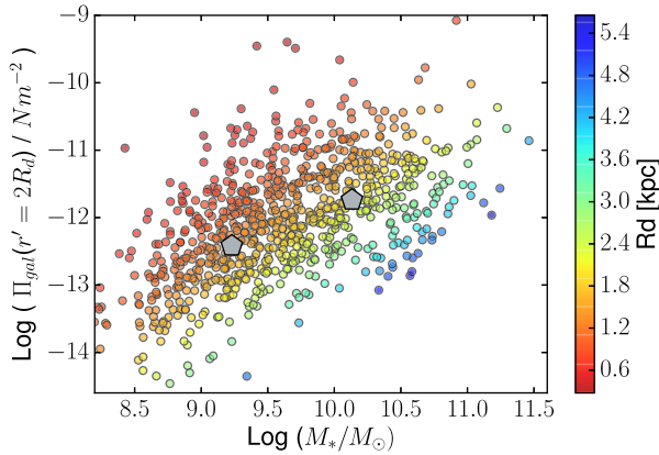
Figure 5. The anchoring force at r' = 2 \times R_d as a function of stellar mass for all spiral galaxies in our (cluster plus field) sample. The grey pentagons correspond to the model galaxies I and II.
