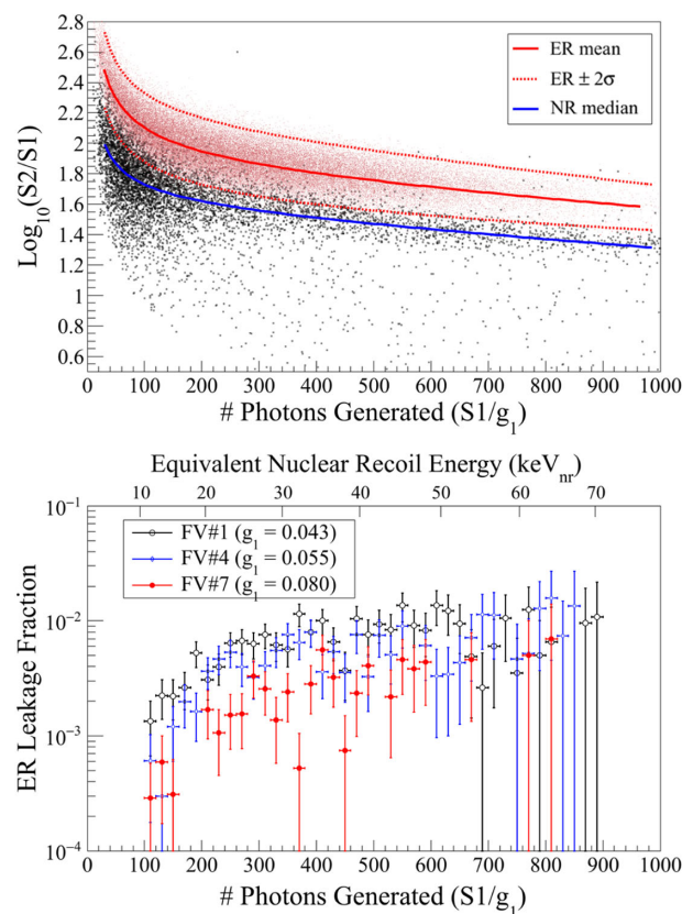
FIG. 9. (Top) ER (red) and NR (gray) bands from the \text{CH}_3\text{T} and ^{241}\text{AmBe} data at 366 V/cm in FV#7, which has the largest value among the seven FVs shown in Fig. 2. The S2 signal is corrected for the electron lifetime. The mean and \pm 2\sigma values of the ER band and the median of the NR band are fit by a power law plus a first order polynomial. (Bottom) The ER leakage fractions obtained by counting the number of events below the NR median, divided by the total number of ER events in each bin, for three different FVs from the top to the bottom of the detector at 366 V/cm drift field. The equivalent nuclear recoil energy is calculated based on the S1 signal following the method in [26].
