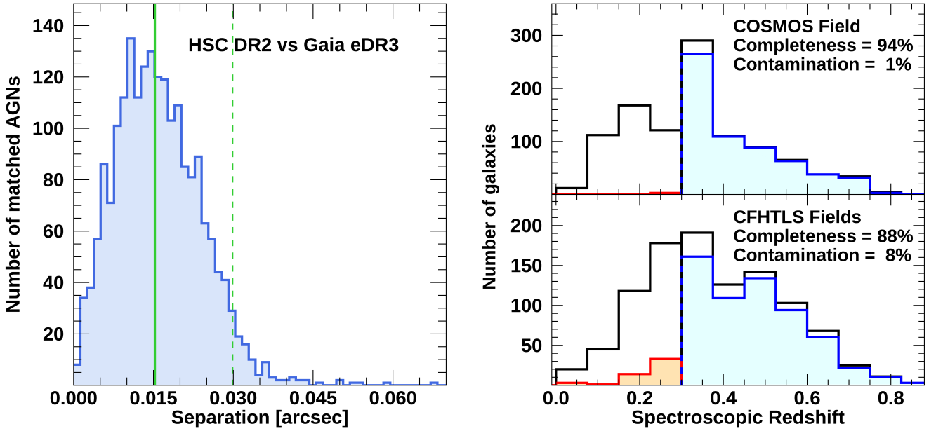
Fig. 5. Astrometric and photometric redshift quality of HSC-SSP data in the four WEAVE-StePS fields. Left panel: histogram of the coordinate cross-match statistics obtained for \sim 2000 matched AGNs, obtained by comparing their Gaia EDR3 and HSC-SSP DR2 coordinates (see text for more details). The median value is the green line at a separation of 0''.015 , and the dashed line is the 95% percentile limit, corresponding to a separation on the sky of \sim 0''.03 . Right panel: completeness and purity of our target selection, estimated using zCOSMOS and VVDS-Wide/Deep spectroscopic data. The top panel shows the COSMOS field, and the bottom panel shows the CFHTLS-W1 and CFHTLS-W2 fields, covered by HSC deep and ultra-deep and HSC wide data, respectively. The histogram outlined in black shows the spectroscopic redshift of all galaxies with a magnitude I_{AB} < 20.5 . The cyan histogram shows the distribution in spec- z of galaxies whose spectroscopic and photometric redshifts, computed using the DEmP algorithm (Hsieh & Yee 2014), are above the 0.3 value redshift cut-off. The orange histogram is the spectroscopic redshift distribution of the subset of galaxies whose photometric redshift is above 0.3 when the corresponding spectroscopic redshift is below this value, as shown by the x -axis. The corresponding values for completeness and contamination of the sample selected using DEmP photometric redshifts are 94/88% and 1/8%, respectively (see text for more details).
