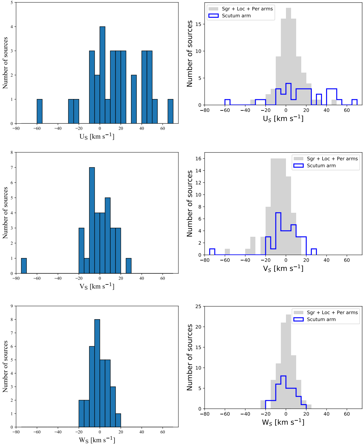
Fig. 3. Distribution of the three peculiar motion vector components U_S ( upper panels ), V_S ( middle panels ), and W_S ( lower panels ) for the Scutum arm sources ( left ) and the combined distribution of the Sagittarius, Local, and Perseus arms sources ( right ) with uncertainties on the peculiar motion components of less than 20 \text{ km s}^{-1} .
