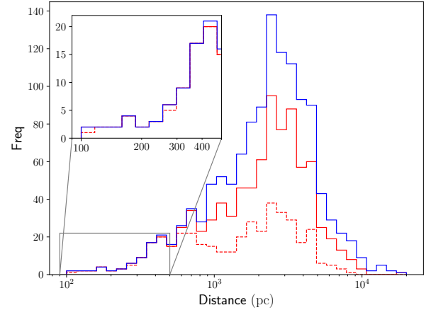
Fig. 6. Histogram of OC distances as listed in Paper I (in blue) for the 861 OCs with a Gaia DR2 RV determination (in red) and for the 406 OCs of the high-quality sample (dotted red). A zoom on nearby OCs is presented in the inset panel.
