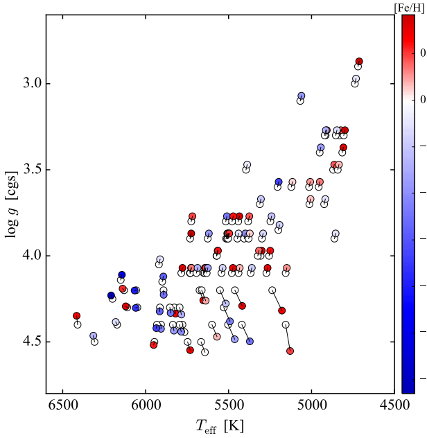
Fig. 4. The empty circles show the stellar parameters before applying the empirical corrections from Bensby et al. (2014) and the coloured circles the parameters after the corrections. The values before and after the corrections are connected with solid lines. On average the effective temperatures change by -9 \pm 12 K and the surface gravities by -0.01 \pm 0.04 . The colours represent [\text{Fe}/\text{H}] , as shown by the colour bar on the right-hand side.
