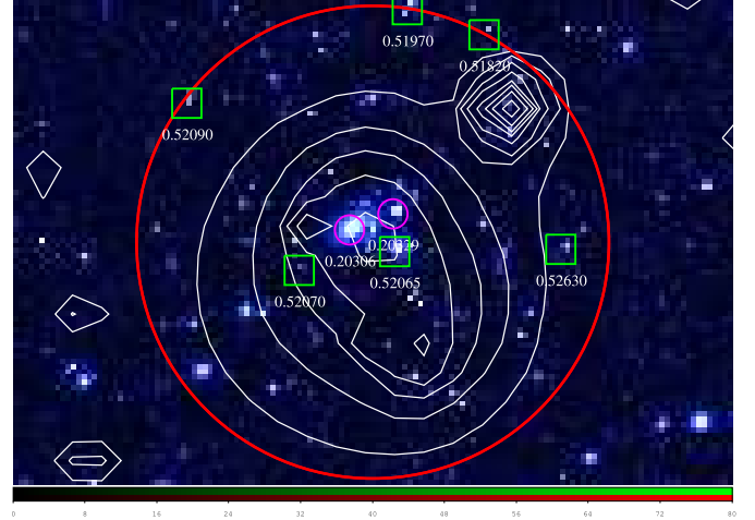
Fig. B.5. CFHTLS i' band 4' \times 2.5' image around XLSSC 096. Green squares represent the member galaxies of the main structure at z = 0.520 and magenta circles are the foreground structure at z = 0.203 . The large red circle represents a 500 kpc radius area. White contours are for the X-ray emission.
