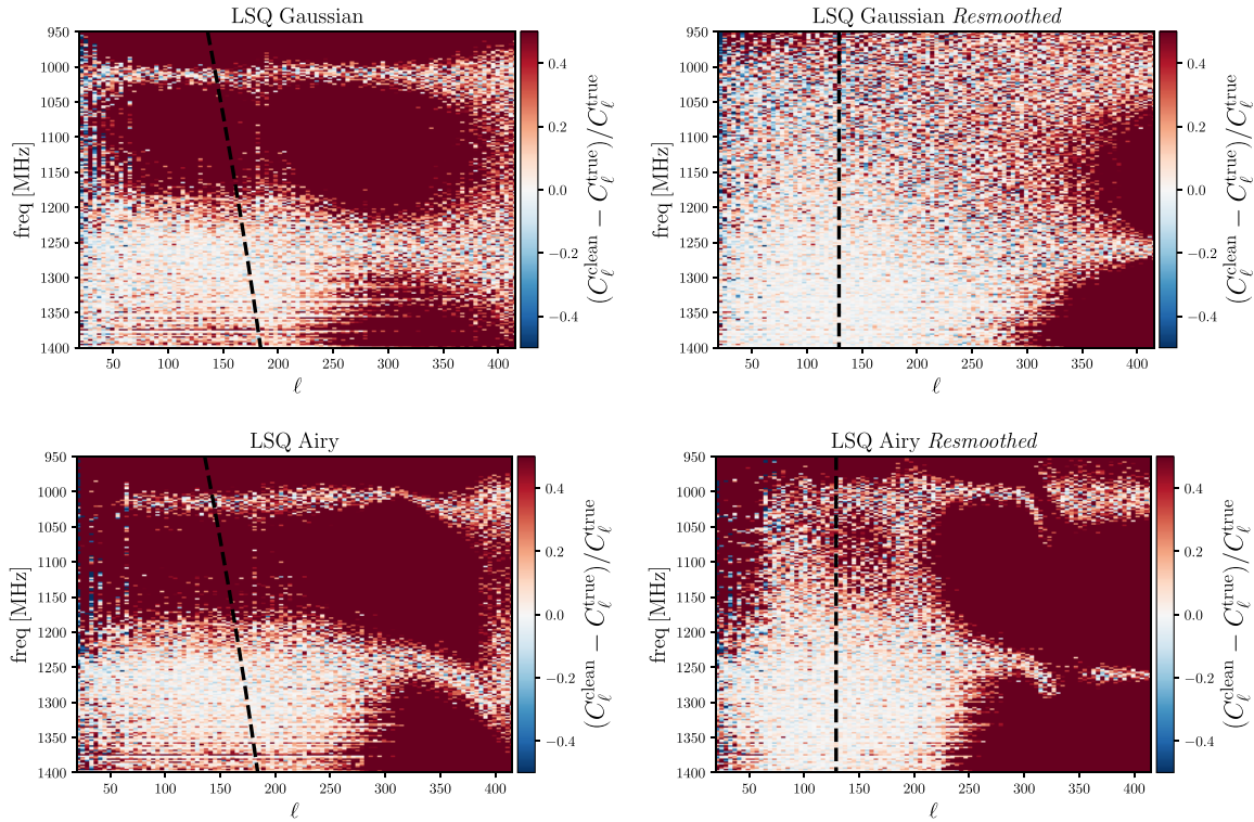
Figure 18. Same as Fig. 17, but here we consider the LSQ method.
