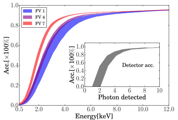
FIG. 5. The signal detection efficiencies in this study for sub-volume 1, 4, 7 as a function of recoil energy are shown in blue, purple and red, respectively. The inset shows the signal detection efficiency from the S1 coincidence requirement (black), which is the dominant contribution to the overall detection efficiency and is a function of detected photon number. The shaded regions represent the 15.4%-84.6% credible region.
