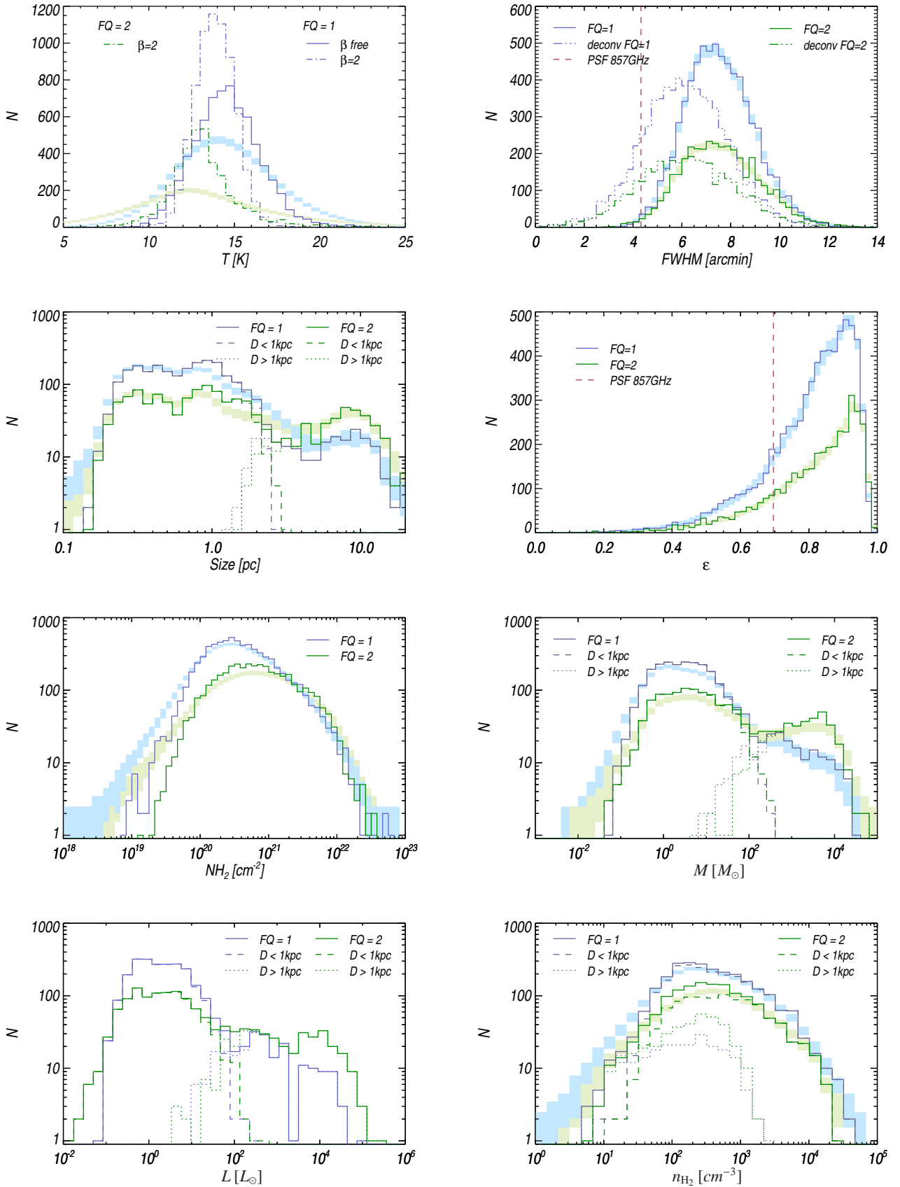
Fig. 11. Distribution of the physical properties of the PGCC objects with FQ=1 (blue) and FQ=2 (green). The coloured shaded regions provide an estimate of the impact of the individual uncertainties on the statistical distribution at a 1\sigma dispersion level around the mean value obtained from 10 000 MC realizations (see Sect. 6 for more details). The temperature distribution is shown for two temperature estimates, i.e., using a free emissivity spectral index \beta (solid line) or a fixed \beta=2 (dot-dashed line). The distribution of the intrinsic size, after deconvolution, is shown on the top right panel in dot-dot-dot-dashed line. The distributions of the physical size, mass, mean density and luminosity of the clumps are provided for sources with reliable distance estimates (DIST_QUALITY=1 or 2). These distributions are also shown separately for sources at solar distances smaller or larger than 1 kpc from the Sun, in dashed and dotted lines, respectively.
