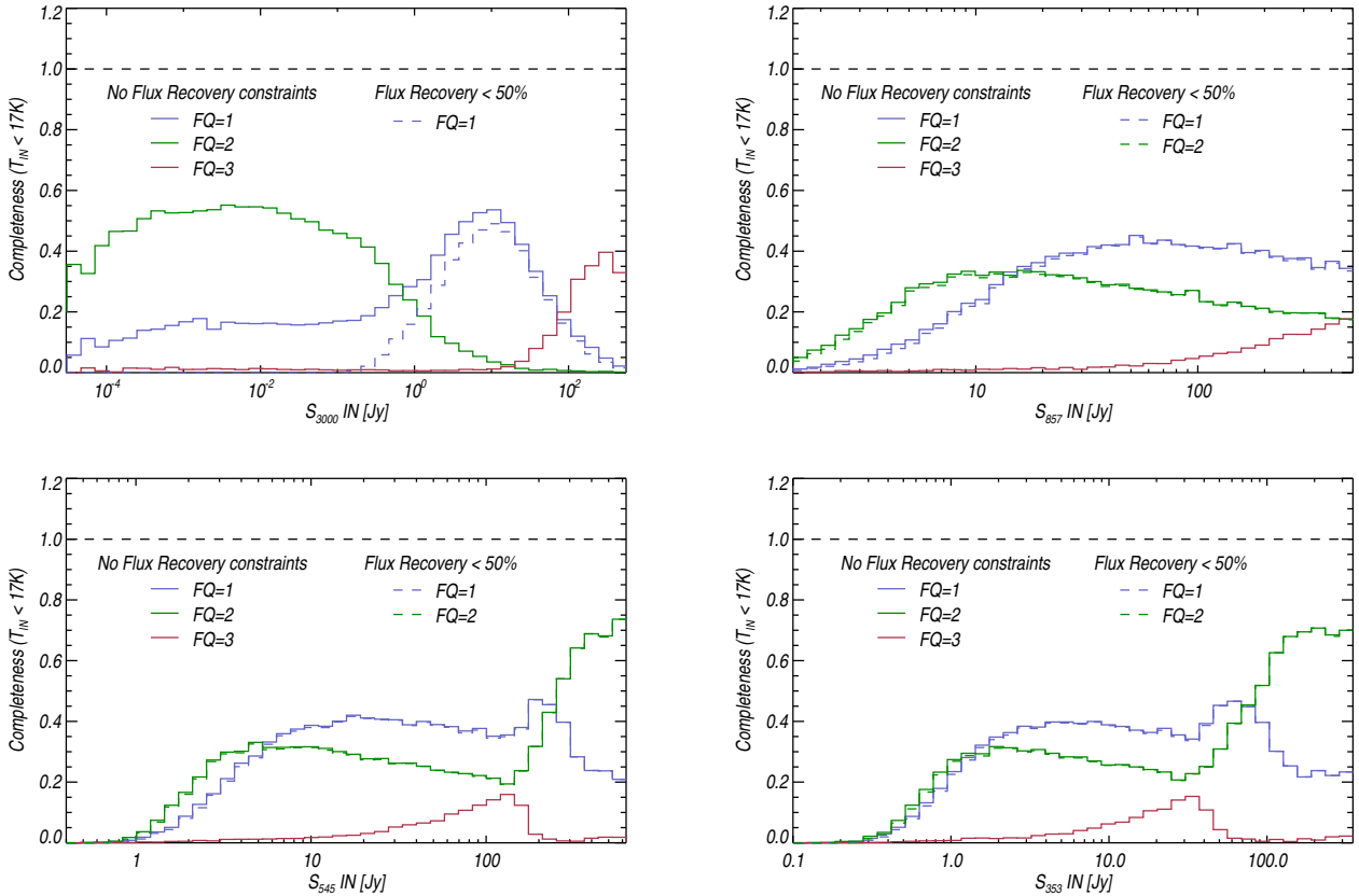
Fig. 4. Completeness (computed on a restricted sample of sources with injected temperature below 17 K) as a function of the injected flux density in the IRAS 3 THz ( top left panel ) and Planck upper frequency bands, 857 GHz ( top right panel ), 545 GHz ( bottom left panel ), and 353 GHz ( bottom right panel ). It is shown per-category of flux density quality, i.e., FQ=1, 2 and 3 categories (blue, green and pink, respectively). The completeness is also computed on a more restricted sample of sources with injected temperature below 17 K and with a flux density accuracy better than 50% ( dashed lines ).
