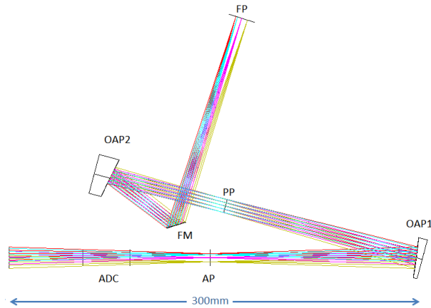
Figure 6: V-SHARK optics layout with labeled its main subsections.
