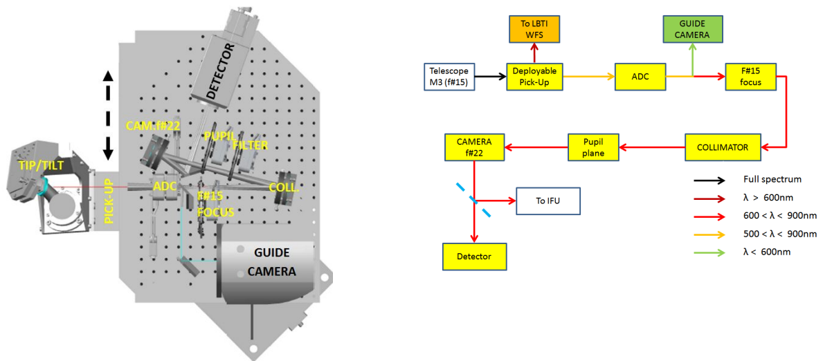
Figure 3. Left: Cad view of the assembly for reference with the system diagram. Right: system level description of V-SHARK architecture with its main functional blocks and light paths. Science path is in red. White modules are not considered parts of V-SHARK.
