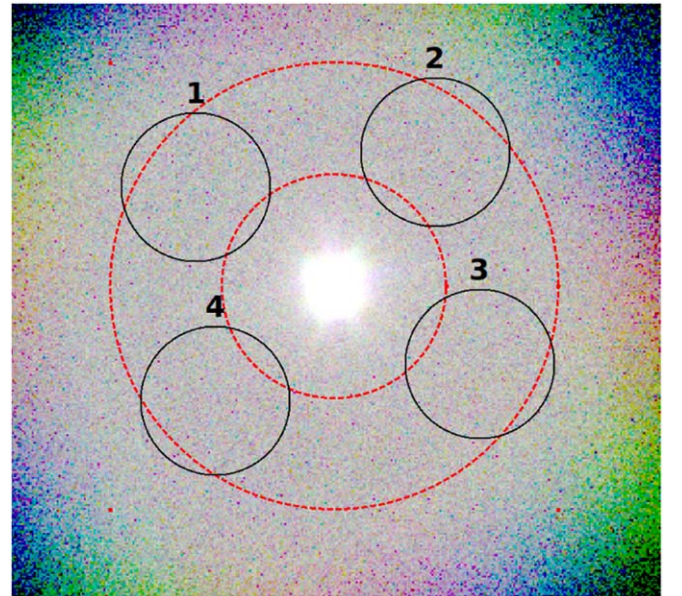
Figure 3. IXPE observation of 4U 0142+61 overimposed with four circular regions, in black, with radius 100'' and an annular region, dotted line in red, with inner radius 2/5 and outer radius 5' . These regions are used to test and compare different background selections in this analysis.
