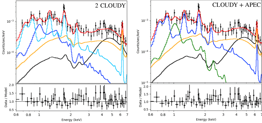
Figure 18. Spectra extracted in the SE sector, best-fit physical models and Data/Model residuals. Models consists of CLOUDY (blue, sky-blue lines), APEC (green, greenlime) and PEXMON (orange) components. The black line is the nuclear spillover plus XBs spectral emission.
