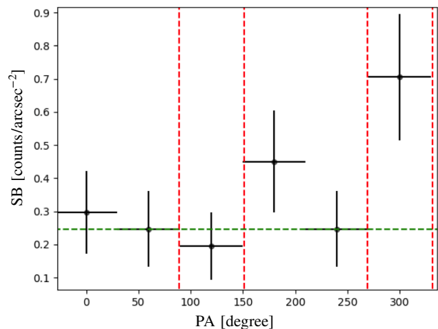
Figure 10. Surface brightness (in counts/arcsec 2 ) azimuthal profile within the 432-840 pc annulus (white annulus in Fig. 9) in the 6.5-6.8 keV image, used as a proxy of the ionized iron line. Red dashed lines separate the bi-cone and cross-cone sectors we consider throughout the paper, while green dashed horizontal line is the average surface brightness estimated excluding the two peak values at 120^\circ and 300^\circ .
