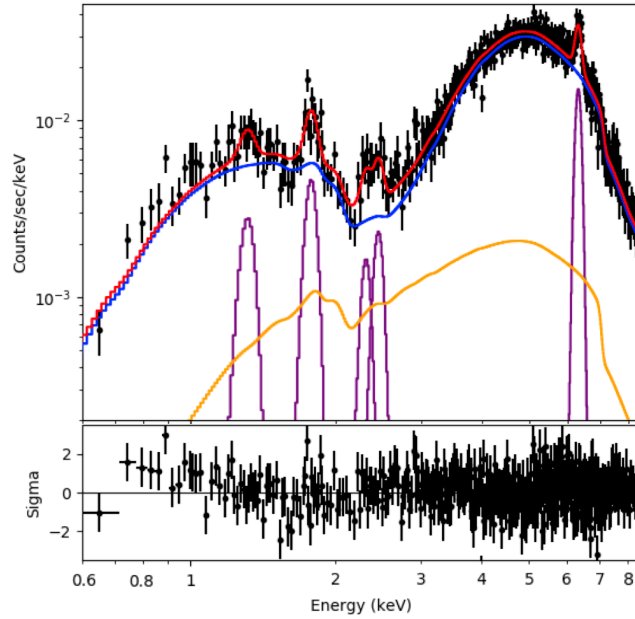
Figure 11. Leaky Absorber fit to the nuclear spectrum of IC 5063 (top panel) and residuals (bottom panel). The spectrum is extracted from a circle of 2'' radius ( \sim 3\text{-}4 PSF) and binned at 20 counts per bin. The total model (red line) includes a partially absorbed power law (blue line), a PEXRAV reflection component (orange line) and five Gaussian lines (purple lines).
