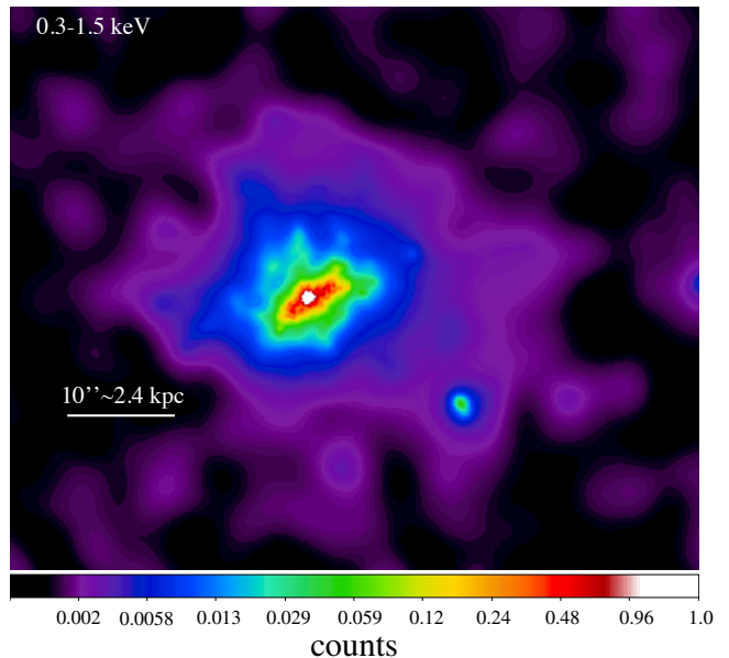
Figure 7. 0.3-1.5 keV image, adaptively smoothed with Gaussian kernels ranging from 0.5 to 30 image pixel (1/8 of instrumental pixel) in 30 iterations and 10 counts under the kernel. The color bar is in counts per image 1/8 subpixel.
