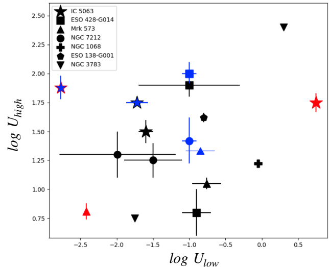
Figure 5. Lower and higher photoionization parameters of the best-fit models obtained for Seyfert galaxies in the literature, compared with our results for IC 5063 (large stars). Nuclear (black); bi-cone (blue); cross-cone (red). The blue stars show a red and a black edge indicating the values for the NW and SE cone, respectively. The blue marks by ESO428-G014 (Fabbiano et al. 2018a) and NGC 7212 (Jones et al. 2020) represent values obtained from the spectral fits in the extended annular region, where, however, the emission along the cones dominates. We included the following Seyferts: Mrk 573 (Paggi et al. 2012), NGC 1068 (Kraemer et al. 2015), ESO-138-G001 (De Cicco et al. 2015) and NGC 3783 (Kaspi et al. 2002; Blustin et al. 2002).
