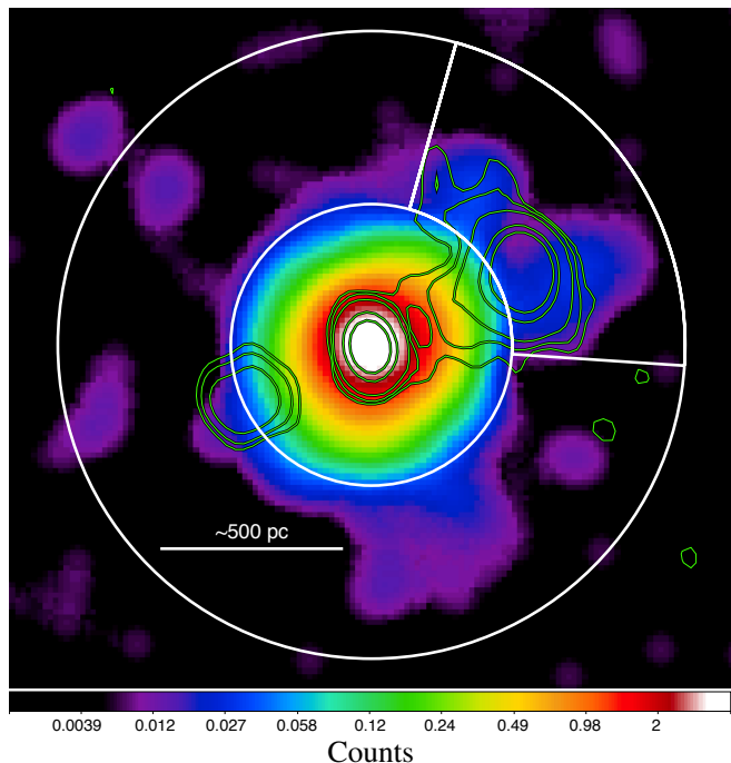
Figure 9. Merged 6.5-6.8 keV image with 1/8 of the ACIS pixel and a Gaussian smoothing with a 10 sub-pixel kernel radius, as a proxy of the ionized iron emission line morphology. In white, we report both the 1.8'' to 3.5'' annulus, and the NW cone sector in which we detect the ionized iron feature at \sim 6.6 keV from the spectral analysis. In green we overlap radio emission contours at 17 GHz and levels 3, 5, 10, 50, 100\sigma (see Fig. 2).
