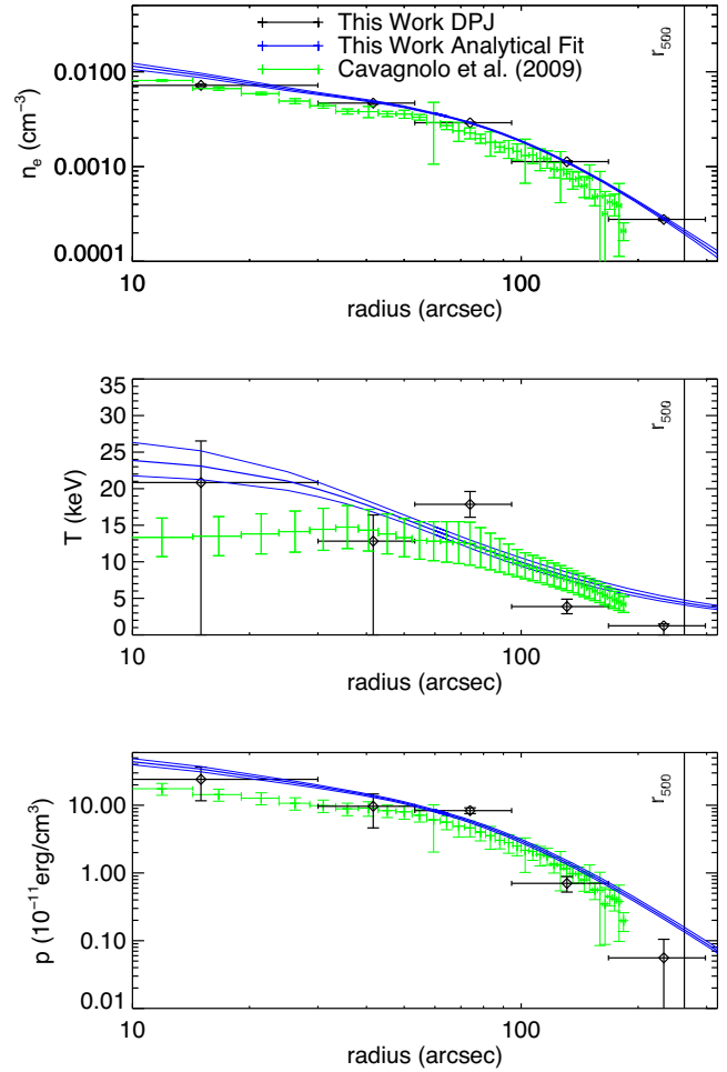
Figure B35. MACS J0717.5+3745 . Our smooth parametric fit indicates a temperature drop at large radii at a significance of 24\sigma . This cluster has been studied extensively in different wavelengths. Ma, Ebeling & Barrett (2009) found that the cluster consists of four large subclusters based on X-ray imaging and galaxy positions. Through lensing (Medezinski et al. 2013; Diego et al. 2015; Limousin et al. 2016; Umetsu et al. 2016), four large masses are also clearly found, reflecting that this cluster is a complex merger. Mroczkowski et al. (2012) studied this cluster through the SZ effect and X-ray and lensing observations. They also found very hot gas near 30 keV in some regions of the cluster. A large kSZ signal in one of the subclusters, which has not been accounted for in our analysis, could potentially be a source of bias in our results (Sayers et al. 2013c).
