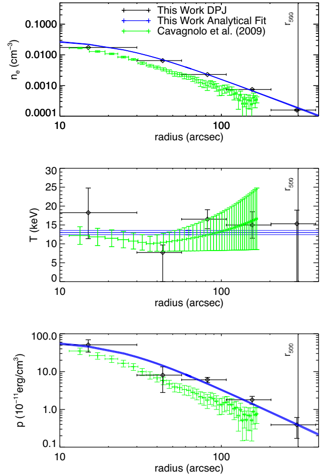
Figure B21. MACS J2211.7–0349 . Our densities and pressures are systematically and significantly higher than those found in the ACCEPT study. Due to the lack of independent results for this cluster, it is not possible to determine which analysis may be in error.
