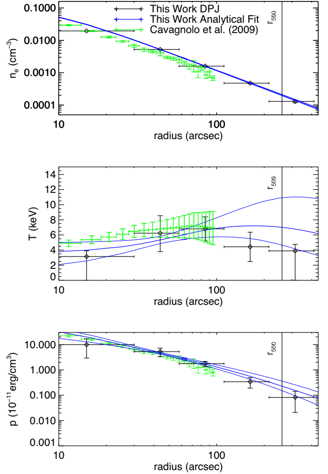
Figure B19. MACSJ1532.9+3021 . Donahue et al. (2014) obtained temperature profiles from X-ray spectroscopy ( XMM-Newton and Chandra ) with the temperature profile showing a central value of 3–4 keV before rising to 8 keV at larger radii, consistent with our analysis. The XMM-Newton profile decreased down to \sim 4 keV at 900 kpc ( \sim 180 arcsec), while the Chandra profile does not show the temperature decrease, instead plateauing at \sim 9 keV. Hlavacek-Larrondo et al. (2013) performed a Chandra , XMM-Newton , VLA, and Hubble analysis. They observed evidence of AGN feedback, a cold front, and X-ray cavities. They note a difference in the temperature map from the east and the west side of the cluster, and find a central temperature of 4 keV rising to 9 keV at 250 kpc ( \sim 50 arcsec). They also detect slight differences in the temperature profile at small radii ( < 25 arcsec) in different directions, with higher temperatures in the S and W directions.
