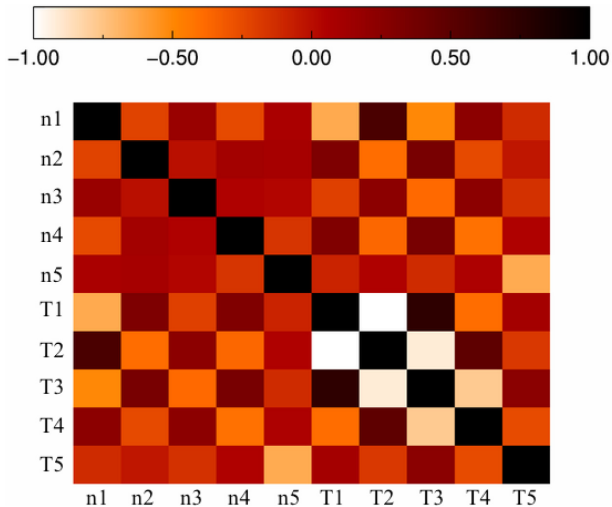
Figure 4. A typical correlation matrix U_k of a concentric shell deprojection (the cluster is MACS J1423.8+2404). n_i denotes the i -th density shell while T_i denotes the i -th temperature shell.
