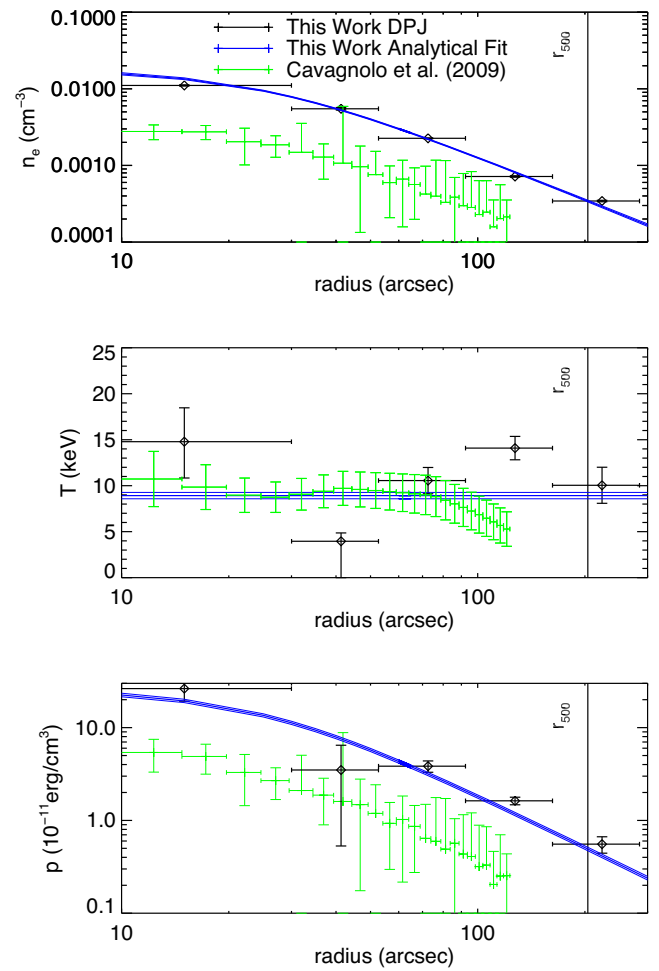
Figure B37. MACS J0454.1-0300 . The densities from the ACCEPT analysis are systematically lower than ours. However, the ACCEPT results are also inconsistent with two other analyses (Bonamente et al. 2006; Amodeo et al. 2016). Donahue et al. (2003) used Chandra X-ray spectroscopy to obtain an isothermal temperature of 10.2 keV, consistent with our results. They also found an elliptical cluster morphology, and a shift in the BCG location and X-ray centroid.
