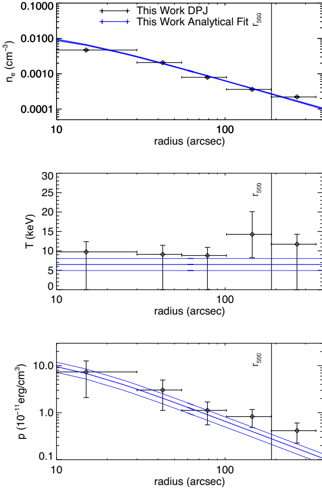
Figure B18. ZWCL 0024+17 . Zhang et al. (2005) performed an XMM-Newton study using imaging and spectroscopy, and found a temperature decrease at large radii (80–180 arcsec) from the isothermal \sim 4 keV central region, which is fairly consistent with our results. They also found an elongation in the X-ray hard ratio map on large scales, and substructure at large radii. Ota et al. (2004) used Chandra spectroscopy and found a nearly isothermal profile of \sim 4.5 keV out to 600 kpc (110 arcsec), again quite similar to our results. Böhringer et al. (2000) used ROSAT to look at the cluster’s X-ray morphology, and found a very small core radius in the surface brightness. They also found an elongation in the X-ray emission; however, it is consistent with a spherical model. Tyson, Kochanski & Dell’Antonio (1998) obtained a mass map using strong lensing measurements, and found a relaxed distribution. Umetsu et al. (2010) performed a full-lensing analysis, including Subaru and Hubble /ACS/NIC3 observations, and looked at X-ray data along with simulations. They suggest that the cluster is in a post-collisional state, with two clusters at the same line of sight, as well as finding the mass profile of the cluster. Jee et al. (2007) noted that the X-ray surface brightness from Chandra is better fitted by two isothermal beta models, suggesting that possibly one could be seeing two systems that are along the same line of sight.
