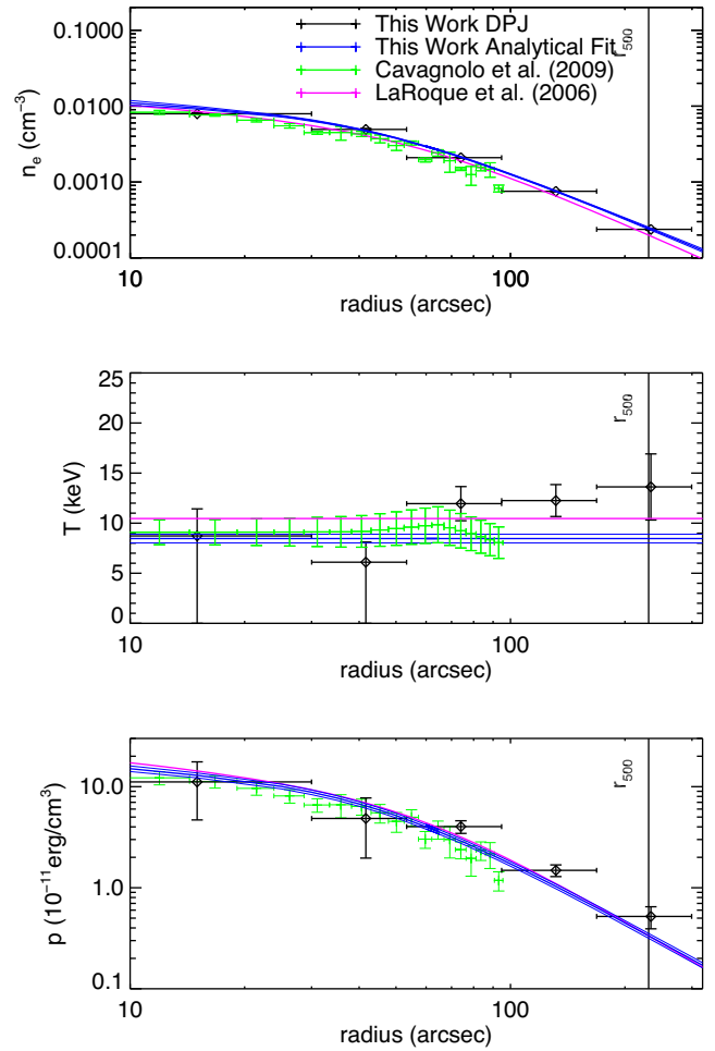
Figure B33. MACS J0018.5+1626 . The profiles we obtain for this cluster are in excellent agreement with the LaRoque et al. (2006) results. Several studies have found this cluster to be relaxed (e.g. Kotov & Vikhlinin 2005), however, Solovyeva et al. (2007) found evidence for it to be undergoing a merger near the centre of the cluster using XMM-Newton observations. They also found a temperature profile out to r_{200} , showing a clear decrease in the outskirts, to 4 keV, which does not match the approximately isothermal profile found in our analysis. Worrall & Birkinshaw (2003) found no evidence of a cool core, but they did find evidence for a merger in the centre of the cluster due to the non-spherical X-ray shape in that region. Overall, they find an isothermal temperature of \sim 9.13 keV, consistent with our results.
