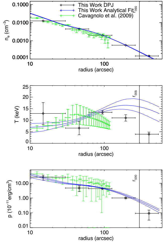
Figure B25. MACS J0417.5-1154 . From our smooth parametric fits, we detect a cool core at a significance of 3.3\sigma . Mann & Ebeling (2012) identified this cluster as a primary candidate for a binary, head-on-collision type merger: The X-ray core aligns with one of two optical cores, but the X-ray emission bleeds into the outskirts and meets with the second of the optical cores.
