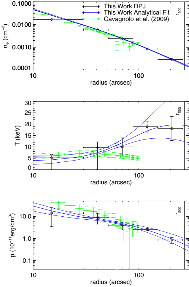
Figure B14. MACS J1931.8–2634 . There is a slight increase in our derived temperatures towards large radii. Based on our smooth parametric fits, there is some evidence of a drop in temperature at the cluster centre ( \sim 2\sigma ). A detailed multiwavelength study of this cluster was performed by Ehlert et al. (2011) using X-ray ( Chandra ), optical ( Subaru ), and radio (Very Large Array) data. They found a cool core with AGN feedback (seen in the X-ray and in the radio), along with evidence of merging, suggesting a cool core that is currently being destroyed. They created a temperature map of the cluster from X-ray spectroscopy out to radii of 500 kpc (100 arcsec), and found an asymmetric temperature distribution. Their azimuthally averaged temperature profile has a central temperature of 5 keV and peak of 10 keV, roughly consistent with our results.
