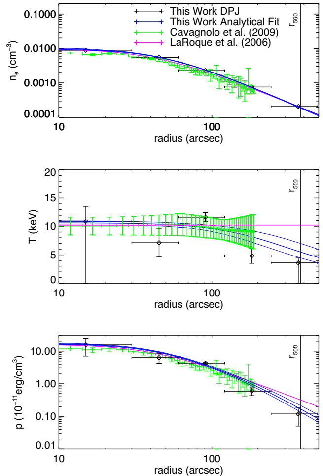
Figure B11. Abell 697. We find a relatively flat inner temperature profile, and we detect a drop in temperature near r_{500} at a significance of 4.5\sigma . Our pressure profiles are consistent with those of the joint X-ray/SZ study of LaRoque et al. (2006). Although we characterized the cluster as non-disturbed, several other studies have shown that the cluster has undergone recent merging. Girardi, Boschini & Barrena (2006) conducted a multiwavelength study using optical and X-ray data, where they calculated line-of-sight galaxy velocity dispersions and spectroscopic temperatures, respectively, and found that A697 is not relaxed. With elongated X-ray emission and substructures near the centre, Abell 697 likely went through many mergers. Through lensing, Metzger & Ma (2000) also concluded that the cluster has undergone a recent merger.
