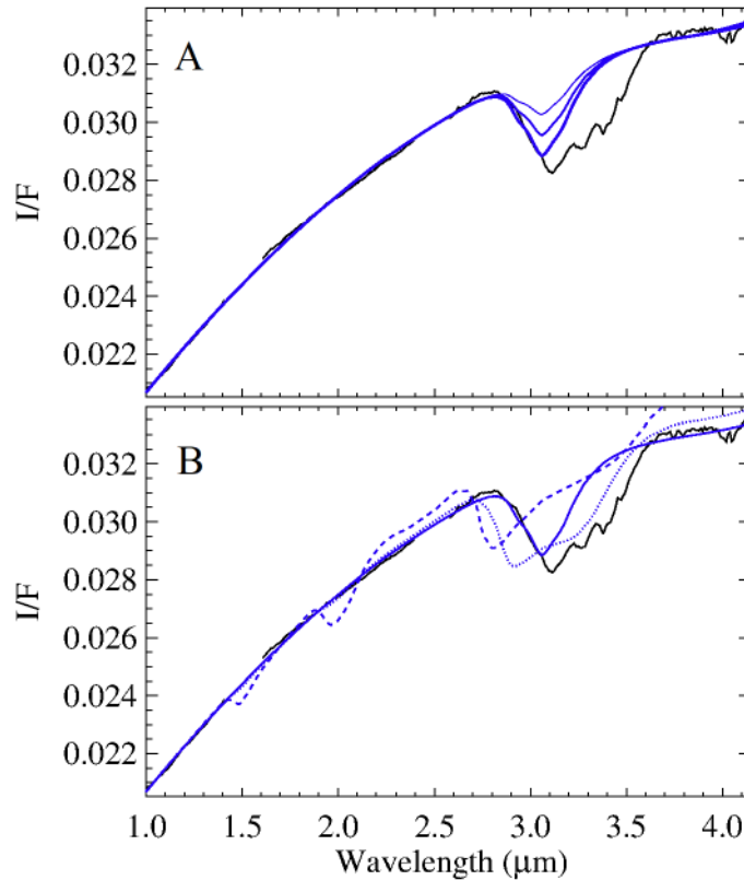
Supplementary Figure 6. Black line: average 67P spectrum; blue lines: modeled water ice mixed with the dark-red endmember. Panel A: water ice grain size fixed at 0.5 \mu\text{m} ; abundance fixed at 1%, 1.5%, and 2% (respectively solid line with increasing thickness). Panel B: water ice abundance fixed at 2%; grain sizes fixed at 0.5 \mu\text{m} (solid line), 5 \mu\text{m} (dotted line), 50 \mu\text{m} (dashed line). We remark that the simulation with particles 0.5 \mu\text{m} -sized is not strictly compatible with a rigorous
