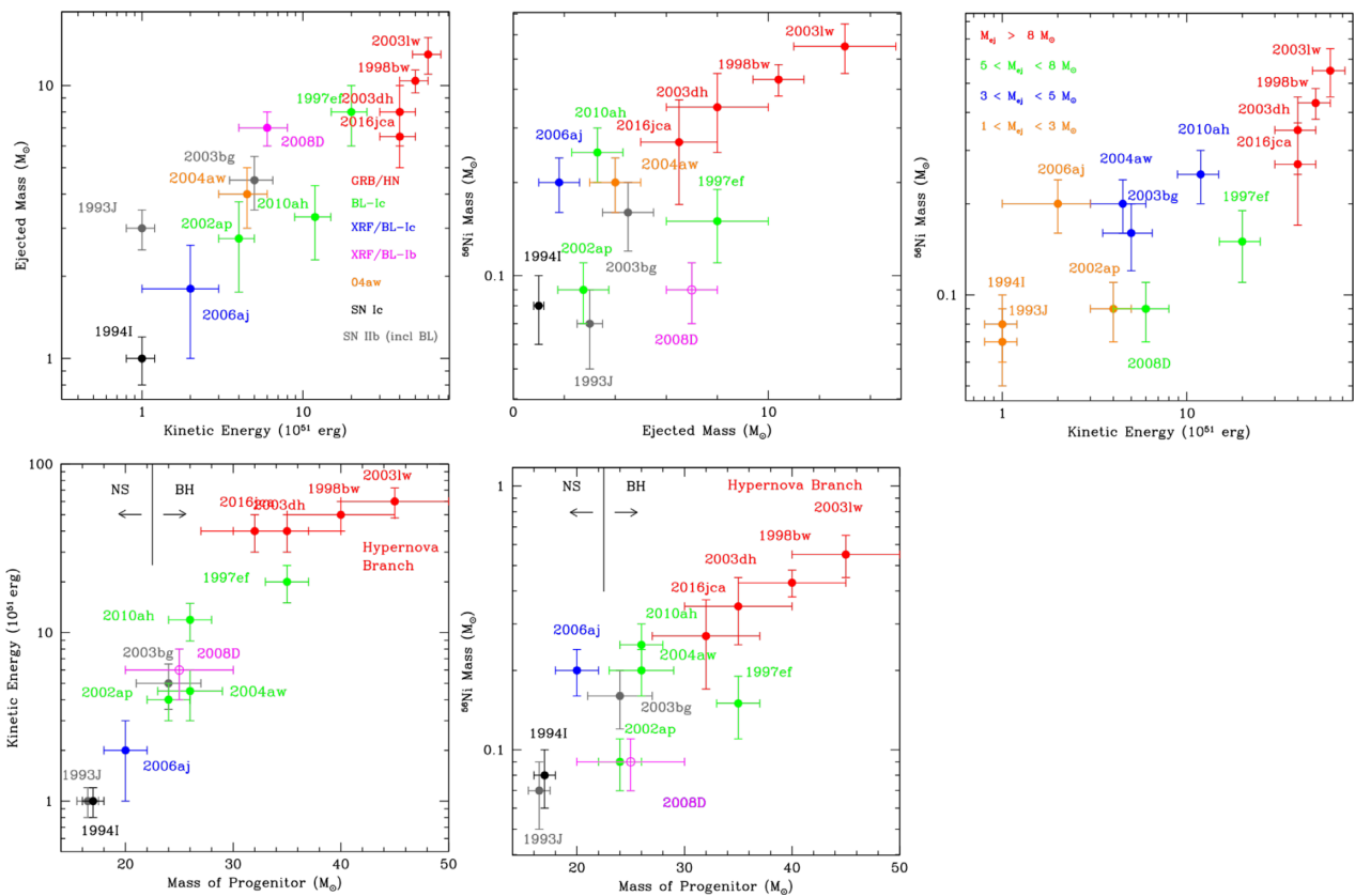
Figure 13. The location of SN 2016jca in terms of the stripped-envelope-SN correlations from Mazzali et al. (2017). For the left and middle panels, the red points are GRB-SNe, the blue points are SNe Ic associated with X-ray flashes, the pink points are SNe Ib associated with X-ray flashes, the black points are normal SNe Ic, and the grey points are normal SNe Iib.
