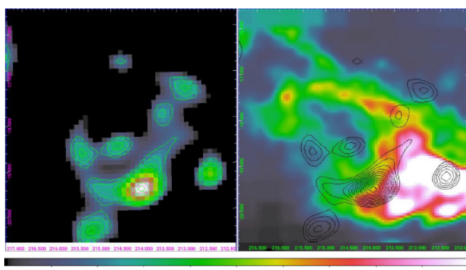
Fig. 6. Left panel: the ring of \gamma -ray excess detected by AGILE. Right panel: the CO map from Dame et al. (2001), which reveals the star forming shell discussed by Pillitteri et al. (2016); the contour levels from the \gamma -ray data are shown in black.
