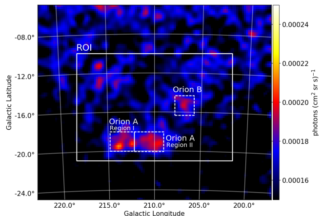
Fig. 1. AGILE map of Orion. The large continuous rectangle highlights the region of interest, over which the best fit model was computed. The dashed rectangles, from left to right, show respectively the subregions 'Region I' and 'Region II' of Orion A, together with Orion B.
