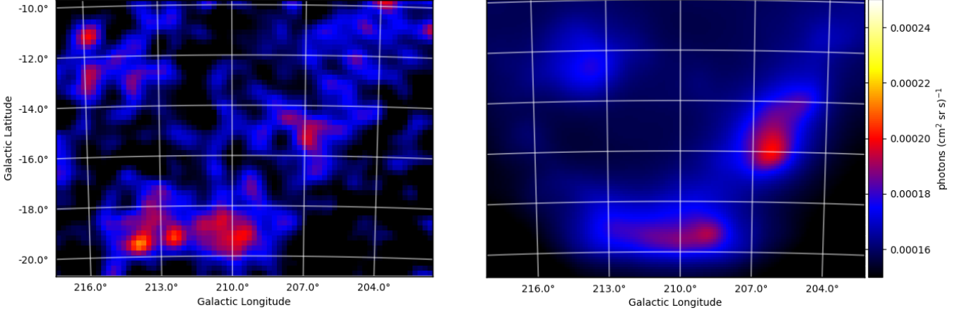
Fig. 2. Comparison between the AGILE (left panel) and the modelled (right panel) maps of the Orion region.
