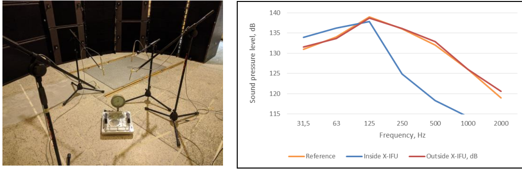
Figure 6. Vacuum tight box used to test the X-IFU filter samples #3 to #7 mounted inside the reverberation chamber at AGH University in Krakow (left panel). The right panel shows the measured sound spectrum inside the reverberation chamber (red line) compared with the reference spectrum (orange line), and the spectrum measured inside the box kept at atmospheric pressure (blue line).
