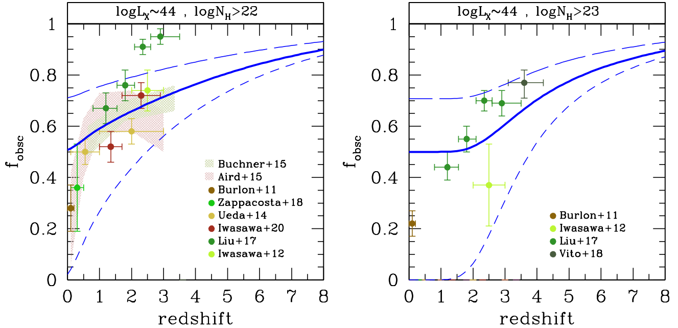
Fig. 14. Total fraction of obscured AGN with \log N_{\text{H}} > 22 (left panel) and \log N_{\text{H}} > 23 (right panel) vs. redshift measured in different X-ray samples (see labels) and compared with model curves of large-scale (ISM) plus small-scale (torus) obscuration. Only samples with median \log L_{\text{X}} \approx 44 have been considered here (see text for details). Curves have the same meaning as in Fig. 13. The model with \gamma = 2 and \theta_{\text{torus}} = 60^\circ (thick solid blue line) provides a good representation of the data.
