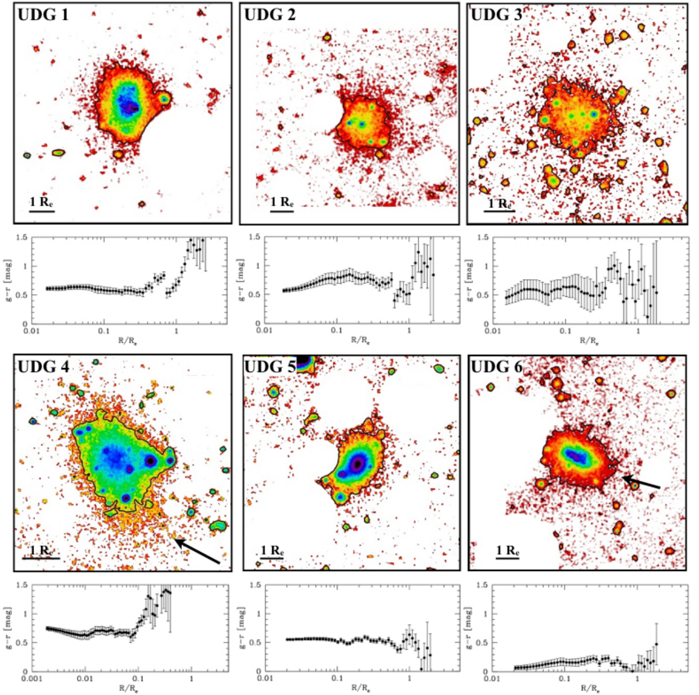
Fig. 2. Images of the UDG candidates in the g band in flux levels. The black contour indicates the surface brightness level of \mu_g = 27 \text{ mag arcsec}^{-2} . In the lower left corner we show the R_e length. The field of view of all boxes is 1 \times 1 \text{ arcmin} ( \sim 14.9 \text{ kpc} ). The black arrow in the image of UDG 4 and UDG 6 indicates the tidal features described in the text. The area that was masked due to contaminating stars is shown as white (circular) background. Below each image we plot the g-r colour profile of the relative UDG.
