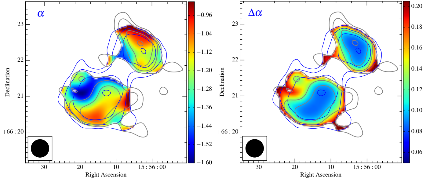
Fig. 3. Left panel: spectral index map between 144 MHz – 1.5 GHz for the extended radio emission from A2146. Right panel: corresponding spectral index error map. The resolution of the maps is 30". In both images, the LOFAR 144 MHz (blue) and VLA 1.5 GHz (grey) first contours are 2.5\sigma , where \sigma = 340 and 27 \mu\text{Jy beam}^{-1} for the LOFAR 144 MHz and VLA 1.5 GHz data, respectively. The next contours are multiplied by \sqrt{3} .
